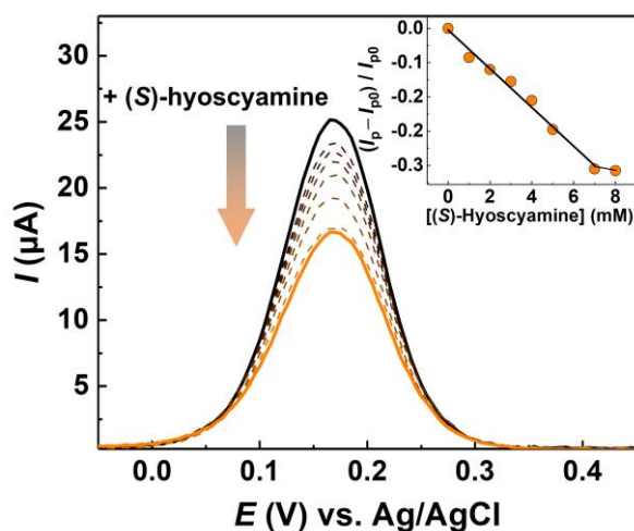
Fig. 4 DPV results of the MIP-AuNS electrode by adding ( S )-hyoscyamine in a phosphate buffer (100 mM, pH 7.0) containing \text{K}_3\text{Fe}(\text{CN})_6 (5 mM) and KCl (100 mM) at 25\text{ }^\circ\text{C} . Inset represents the ratio of the peak current ( I_p ) changes of the MIP-AuNS electrode. The terms I_{p0} and I_p indicate the peak current before and after adding ( S )-hyoscyamine, respectively. [(\text{S})\text{-Hyoscyamine}] = 0.0\text{--}8.0\text{ mM} .
