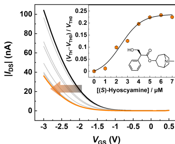
Fig. 5 Transfer characteristics of the MIP-OFET upon the addition of ( S )-hyoscyamine in a phosphate buffer (100 mM, pH 7.0) containing KCl (100 mM) at 25\text{ }^\circ\text{C} . Inset represents the titration isotherm corresponding to the ( S )-hyoscyamine induced V_{\text{th}} shift. [(\text{S})\text{-Hyoscyamine}] = 0.0\text{--}7.0\text{ }\mu\text{M} .
