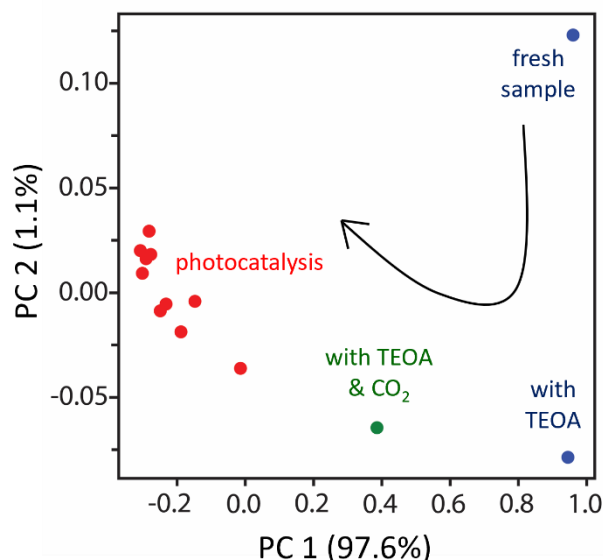
Figure 4. Plot of 1 st and 2 nd PCA components of each XANES spectra followed by a K-means clustering (different colours represent different clusters). PC 1 accounts for 97.6% of the total variation around all the spectra, and PC 2 accounts for 1.11%.
