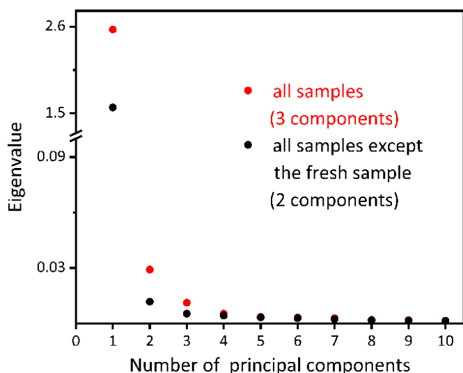
Figure 3. PCA scree plot showing the result from two set of XANES spectra, one of all the samples (red) and another one of all the sample except the fresh sample.
