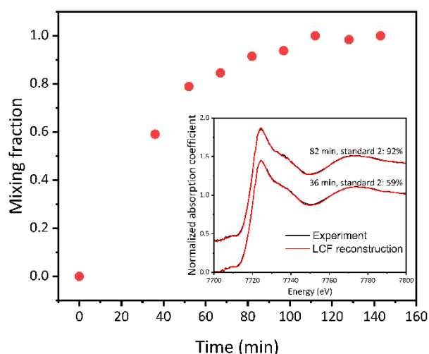
Figure 5. Linear combination fitting results showing the obtained mixing fraction of standard two. Standard one is the sample with TEOA and CO 2 purge before light. Standard two is the sample with light on for 143 min for reaction. Inset shows a comparison between the experimental XANES spectrum and the corresponding reconstruction of XANES spectrum from LCF result at 2 different reaction times.
