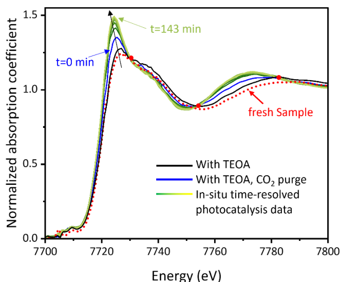
Figure 2. XANES spectra of the samples during the photocatalysis reaction including the fresh sample and the ones after the reaction.
