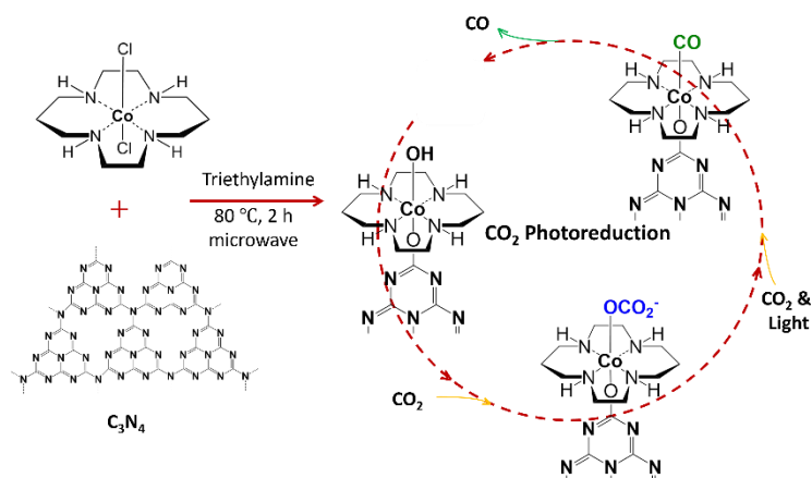
Figure 1. Schematic representation showing the synthesis of Co-cyclam/ C_3N_4 and possible intermediates in photoreduction of CO_2 using the prepared catalyst in the presence of a sacrificial electron donor, triethanolamine (TEOA).
