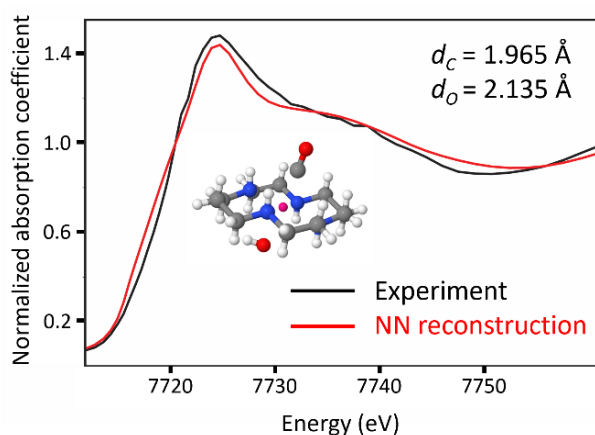
Figure 10. The comparison of the experimental XANES spectra (black) and the theoretical XANES spectra reconstructed from the descriptors values predicted from NN.
