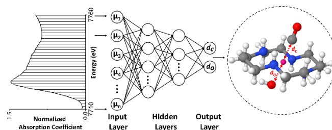
Figure 7. A schematic that represents the application of NN-XANES to SACs system of Co-cyclam-CO.
