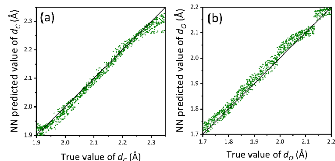
Figure 9. Prediction accuracy of the NN models on the test dataset. a) d_C versus predicted d_C (Å), b) d_O versus predicted d_O (Å).
