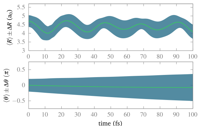
Fig. 4 Time evolution of the expected bond length \langle R(t) \rangle , the expected angle between the field \mathbf{E}_1 and the molecular axis \langle \theta(t) \rangle , and their corresponding standard deviations, in the presence of a circularly polarized field with \omega = 0.1 a.u., E_1 = E_2 = 0.02 a.u. The initial wave function corresponds to a Gaussian in R displaced 0.5 a_0 from R_0 , times a Gaussian in \theta with \sigma_\theta = 0.2\pi .
