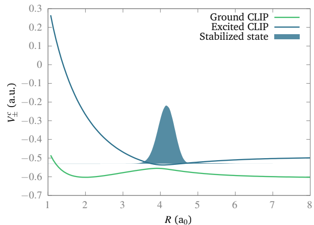
Fig. 2 Ground and excited light-induced potentials prepared by a strong field of circular polarization (CLIPs) with \omega = 0.1 a.u. and E_1 = E_2 = 0.02 a.u. as a function of the internuclear distance. The curves do not depend on \theta . Also shown is the ground vibrational wavefunction in the excited CLIP. Note that the CLIPs exhibit bond hardening, bond softening and an avoided crossing for all values of the angle.
