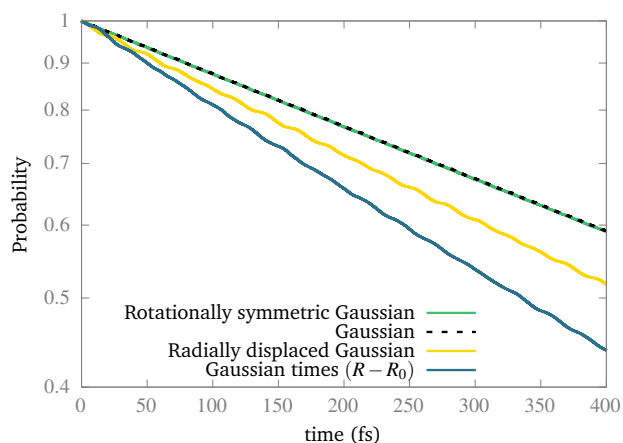
Fig. 3 Population decay in the presence of a circularly polarized field for a set of different initial wave packets initially prepared in V_+^c , measured as the norm of the wave function in the grid.
