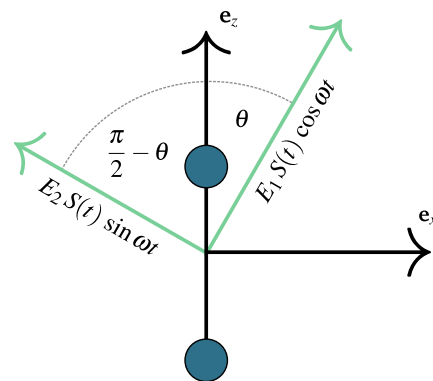
Fig. 1 Diagram of H 2 + molecule under an elliptically polarized field. The field can be understood as two perpendicular linearly polarized fields with different amplitudes that differ in phase by \pi/2 .
