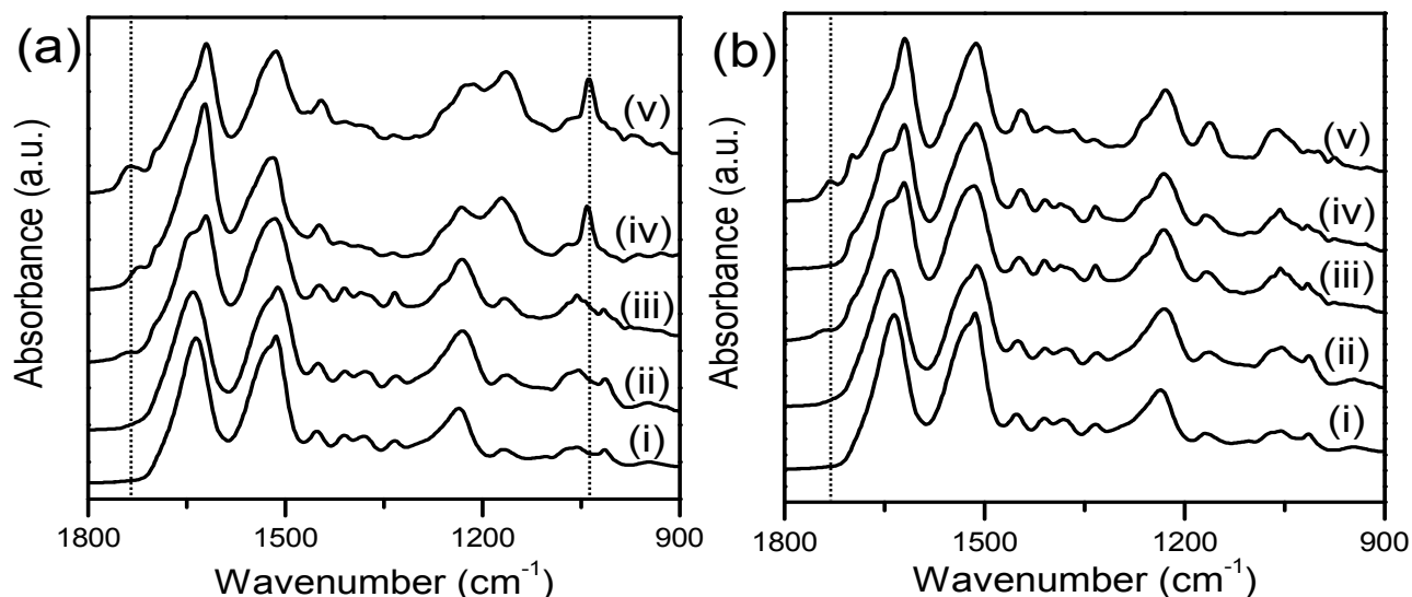
Figure 1. (a) ATR-FTIR spectra of (i) Unmodified SF ( SF_{As\ Cast} ), (ii) SF_{EO} , (iii) SF_{OX} , (iv) SF_{EO} -zwitter, (v) SF_{OX} -zwitter, and (b) ATR-FTIR spectra of (i) Unmodified SF ( SF_{As\ Cast} ), (ii) SF_{EO} , (iii) SF_{OX} , (iv) SF_{EO} -PEG, (v) SF_{OX} -PEG. Vertical dashed reference lines in (a) correspond to S=O stretching at 1040\text{ cm}^{-1} and ester C=O stretching at 1735\text{ cm}^{-1} , and the dashed reference line in (b) corresponds to ester C=O stretching at 1735\text{ cm}^{-1} .
