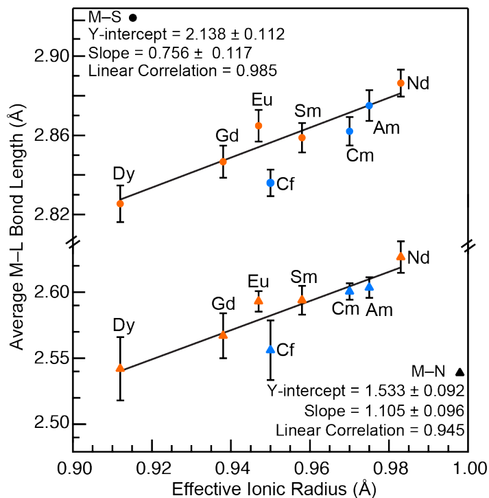
Figure 2. Comparison of the mean M–S (●; top ) and M–N (▲; bottom ) bond lengths in M(\text{S}_2\text{CNEt}_2)_3(\text{N}_2\text{C}_{12}\text{H}_8) ( M = \text{Nd}, \text{Sm}, \text{Eu}, \text{Gd}, \text{Dy}, \text{Am}, \text{Cm}, and \text{Cf} ) versus six-coordinate metal ionic radii. 11, 12, 17 Lanthanides are represented by orange symbols and actinides by blue symbols. Uncertainty is reported as standard deviation from the mean ( 1\sigma ). Data were fit with a line ( y = mx + b ), as shown by the solid black trace.
