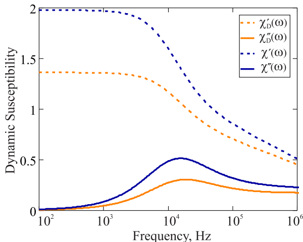
Fig. 1 Dynamic Susceptibility 4\pi\chi(\omega) of F1: comparison of the Debye ideal gas model to the expressions in Eq. (18). Frequency range is given in log-scale. Here, \phi_m = 0.06 ; T = 293 K; K = 20 kJ/m 3 ; effective viscosity \eta = 2 \times 10^3 Pa sec; M_0 = 480 kA/m.
