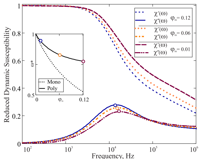
Fig. 2 Reduced Dynamic Susceptibility \chi(\omega)/\chi(0) of F1: the effect of dilution. Three spectrums are plotted for \phi_m = 0.12; 0.06; 0.01 in blue, orange and bordeaux respectively. Frequency range is given in log-scale. Inset: the dependence \omega^*(\phi_m)/\omega^*(0) . Solid line is the solution of Eq. (21); the dotted line is a corresponding monodisperse sample Eq. (23).
