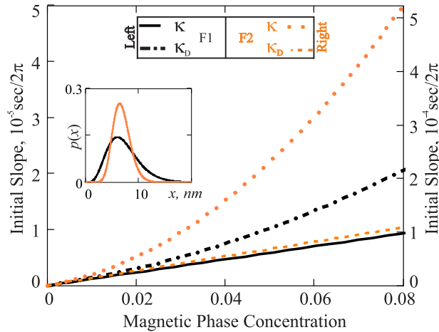
Fig. 4 Initial slope ( \kappa ) as a function of \phi_m : comparison of the Debye ideal gas model to the expressions in Eq. (25). The results for F1 (black) are associated with the left ordinate axis; the results for F2 (orange) with the right one. Inset: particle size distributions versus magnetic core diameter ( x ).
