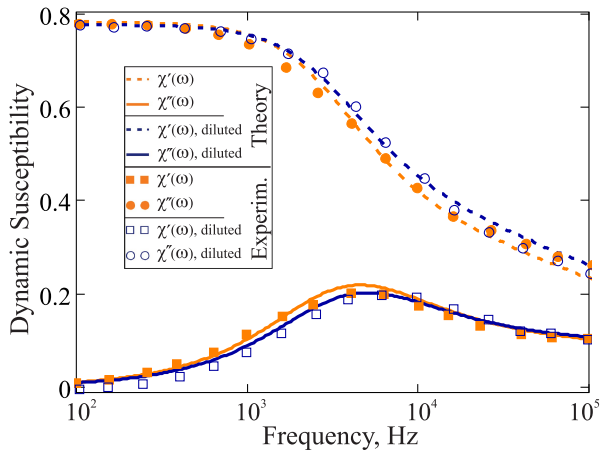
Fig. 3 Dynamic Susceptibility 4\pi\chi(\omega) of F2: comparison of the experimental data to the expressions in Eq. (18). Frequency range is given in log-scale. Here, mass fraction of iron for the basic sample is 0.061; T = 293 K; K = 100 kJ/m 3 ; effective viscosity \eta = 5 \times 10^3 Pa sec; M_0 = 1490 kA/m. Reference sample: orange, filled symbols; 10 times diluted sample: blue, empty symbols (rescaled to be visible).
