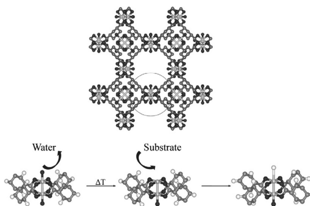
Fig. 2 HKUST-1 porous structure (top) Cu_2 Paddle-wheel showing terminal water molecules, thermal activation affords Lewis site by water removal allowing substrate activation on the vacancy from ref. 31.
