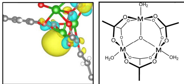
Fig. 3 Lewis sites: metal trimer showing water molecules as labile ligand (right) and volume of the orbital of Ni of CPO-27 (MOF-74) as calculated by DFT from ref. 41 (left).
