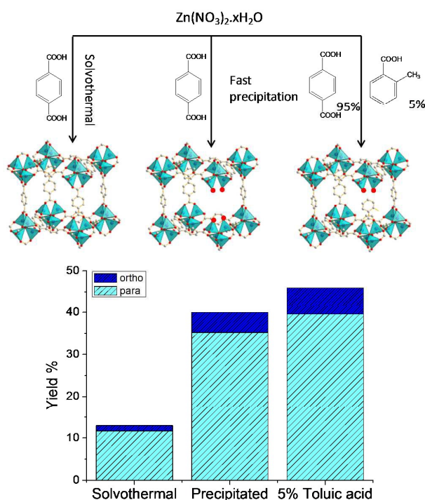
Fig. 11 Synthesis of defective MOF-5 by fast precipitation and using dummy linker. Comparison of catalytic performances on the benzylation of toluene by comparison with a solvothermal process sample from ref. 78.
