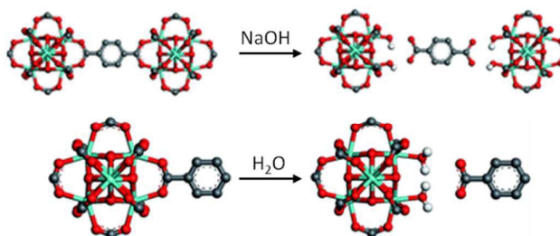
Fig. 9 Proposed ligand displacement mechanism for UiO-66 breakdown in presence of sodium hydroxide or water. Reprinted with permission from ref. 76.
