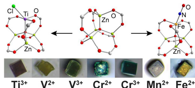
Fig. 13 Isomorphous substitution of \text{Zn}^{2+} by other metal cations at the \text{Zn}_4\text{O} cornerstone of MOF-5 from ref. 85.
