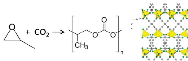
Fig. 8 Propylene oxide and CO 2 copolymerization catalysed by layered structure of zinc glutarate from ref. 74.
