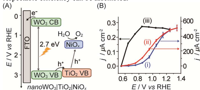
Fig. 11. (A) Schematic energy diagram of \text{nanoWO}_3|\text{TiO}_2|\text{NiO}_x for visible light-driven water oxidation (hole transfer from \text{WO}_3 directly to \text{NiO}_x is also possible) 36 and (B) photocurrent responses of (i) \text{nanoWO}_3 , (ii) \text{nanoWO}_3|\text{TiO}_2 , and (iii) \text{mesoITO}|\text{PSII} electrodes under standardised solar light irradiation (AM 1.5G, 100 \text{mW cm}^{-2} ; Y.-H. Lai, M. Kato, E. Reisner, manuscript in preparation). Photocurrents for (i) and (ii) were recorded in an aqueous potassium borate buffered solution (0.1 M, pH 9.2) and for (iii) in a MES buffer solution (0.04 M, pH 6.5). Photocurrents are plotted against the reversed hydrogen electrode (RHE) and RHE can be converted to NHE by adding -0.059 \times \text{pH} .
