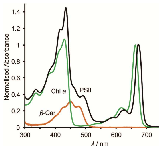
Fig. 2 UV-visible absorption spectra of Chl a (in methanol, green trace), \beta -carotenoid (in hexane, orange trace) and PSII (in MES buffer, black trace). Traces were taken from Frigaard et al. FEMS Microbiol. Ecol. , 1996, 20 , 69–77; Zechmeister and Polgar J. Am. Chem. Soc. , 1943, 65 , 1522–1528. The spectra have been normalised to the value of 1 at the peaks corresponding to the Chl a band at 670\text{ nm} and \beta -carotenoid at its 450\text{ nm} absorption band. The \beta -carotenoid spectrum was then scaled down by a factor of 11/35 to reflect the carotenoid to Chl molecular ratio per PSII monomer.
