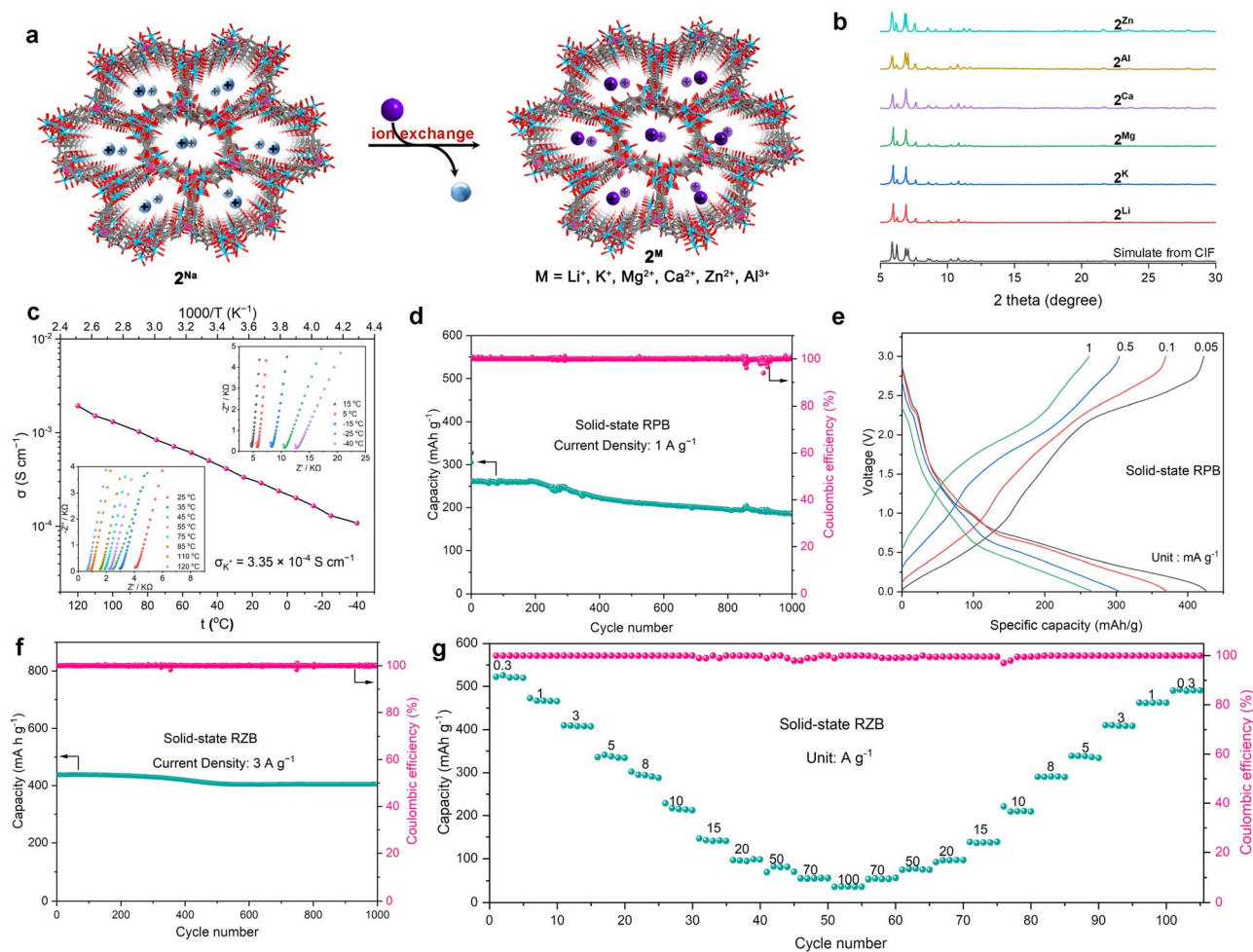
Fig. 4 (a) Schematic illustration of tetraphenylborate-based anionic MOFs as a versatile single-ion conductor through ion-exchange. (b) PXRD patterns of 2^M , M = \text{Li, K, Mg, Ca, Zn, and Al} . (c) Ionic conductivity of 2^K as a function of temperature in the range from -40 to 120 °C. Inset: Nyquist plots for 2^K . (d) Long-term GCD performance of the RPB at 1 \text{ A g}^{-1} . (e) Rate performance of the RPB at current densities from 0.05 to 1 \text{ A g}^{-1} at room temperature. (f) Long-term GCD performance of the RZB at 3 \text{ A g}^{-1} . (g) Rate and cycling performance of the RZB at current densities from 0.3 to 100 \text{ A g}^{-1} at room temperature.
