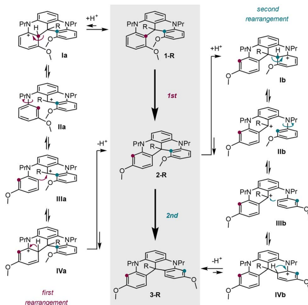
Scheme 3 Acid-mediated transformation of 1-R into 2-R and 3-R (central column, R = H or Me). Mechanistic rationale for first (left) and second (right) skeletal rearrangements.
