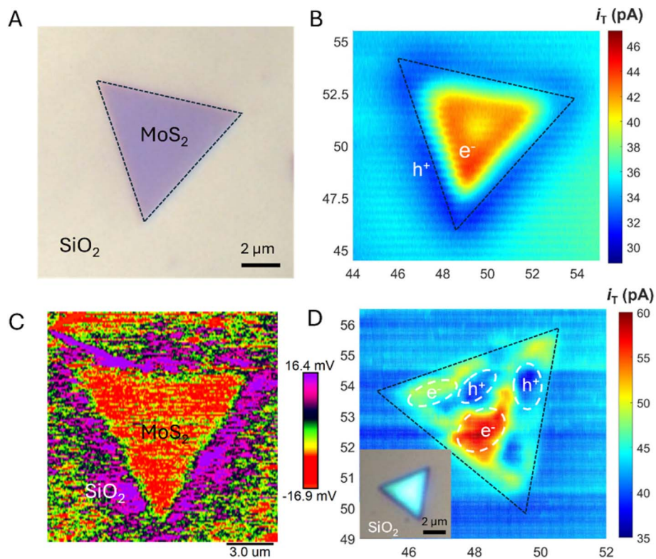
Fig. 11 (A) Optical micrograph of a few-layer thick \text{MoS}_2 triangle. (B) Constant-height photo-SECM image of the same triangle. (C) SPVM image of the few-layer thick \text{MoS}_2 triangle on a \text{SiO}_2 support in air. (D) Photo-SECM image of the bulk \text{MoS}_2 triangle on a \text{SiO}_2 support. Reproduced from ref. 46 with permission from American Chemical Society, copyright 2025.
