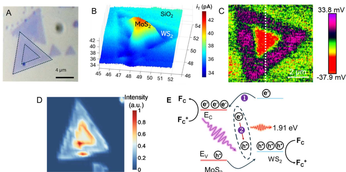
Fig. 12 Optical micrograph (A), constant-height photo-SECM image (B), SPVM image (C), and PL image (D) of in-plane \text{WS}_2 - \text{MoS}_2 heterojunctions. (E) Proposed energy band diagram of the heterojunction. Reproduced from ref. 84 with permission from American Chemical Society, copyright 2026.
