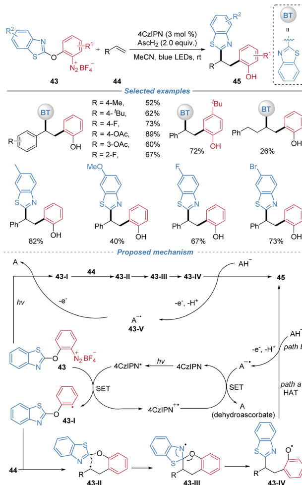
Scheme 16 Intermolecular radical difunctionalization by docking-migration of arylbenzothiazolyloether reagents.
