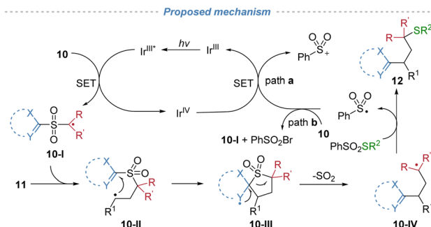
Scheme 5 Polarity-umpoling three-component radical alkylation of alkenes.
