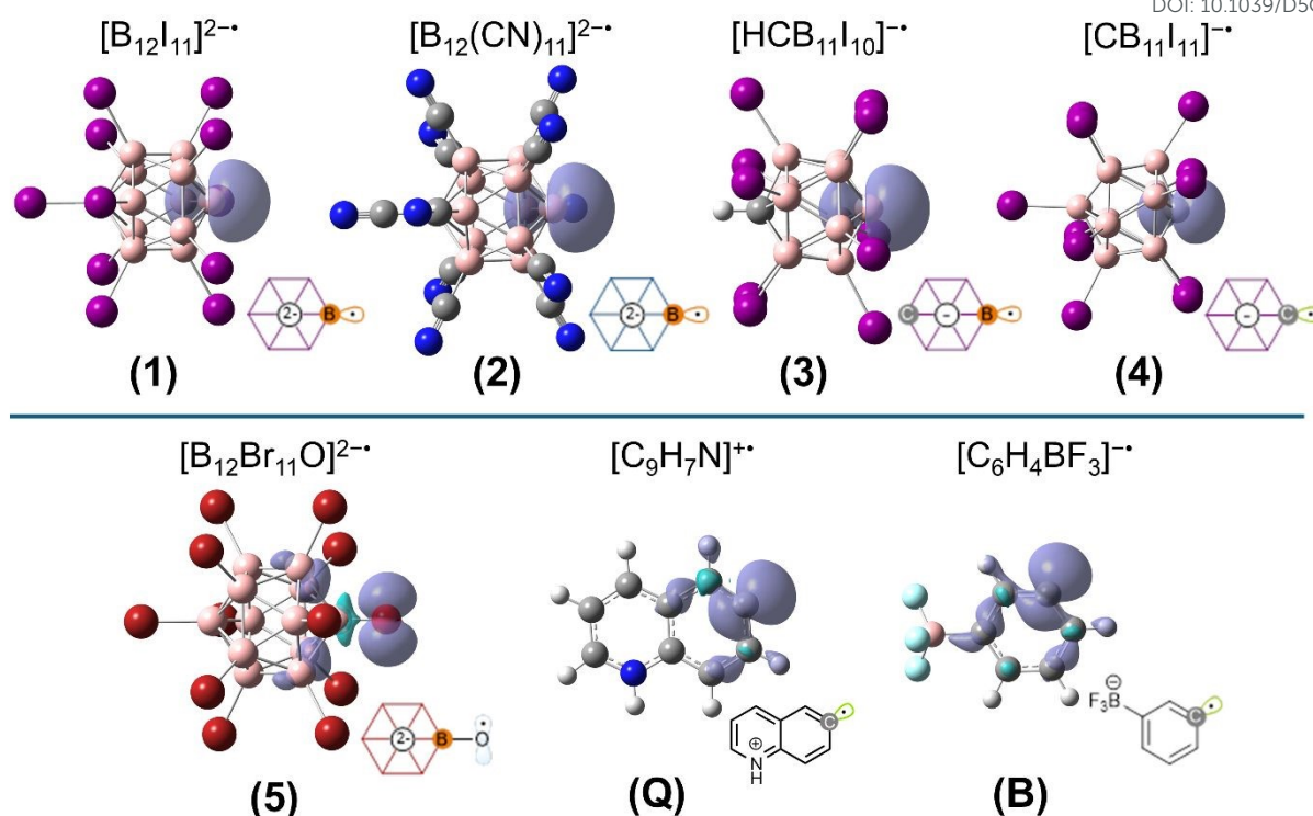
Figure 2: DFT-calculated optimized geometries and semi-transparent isosurface representations of the spin density (a-b spin) of the five closo -borate radical anion derivatives 1-5 and the two organic radical ions Q and B investigated in this study. Isosurface representations are displayed at an isovalue of 0.003. At the bottom right of each geometry, a pictogram is introduced, which will be used throughout the results section to signify the respective radical ions.
