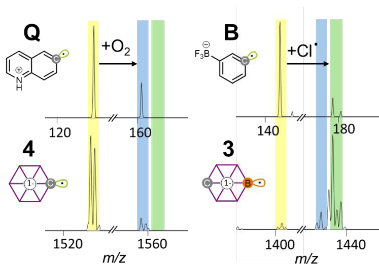
Figure 5: Mass spectra obtained after 1000 ms reaction between isolated ions Q , B , 4 and 3 with carbon tetrachloride in the ion trap of a linear quadrupole ion trap mass spectrometer. The ion trap also contained ubiquitous residual \text{O}_2 gas. The signal of the isolated radical ion is marked yellow. Ions B and 3 react with carbon tetrachloride to form the \text{Cl}^\bullet abstraction product ions (marked in green). Binding with residual \text{O}_2 gas is marked in blue. The mass spectra obtained after 1000 ms reaction time between isolated ions 1 and 2 with \text{CCl}_4 are shown in Figure S9.
