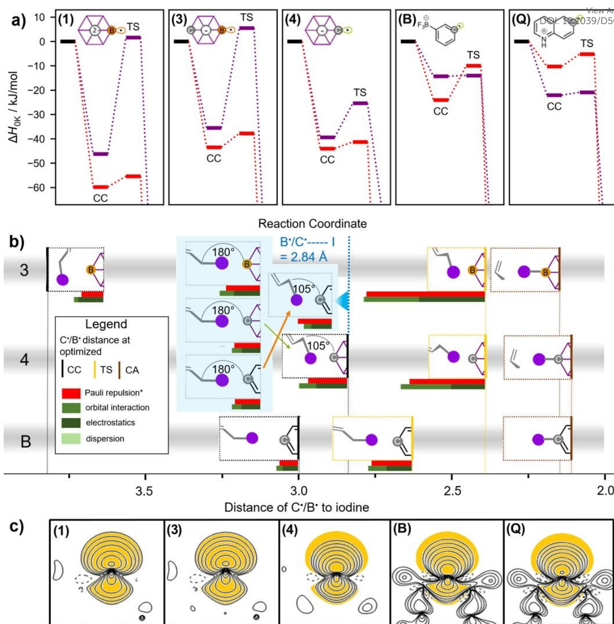
Figure 7: a) PES diagrams (M06-2X-D3/def2-TZVPP) for binding of ions 1 , 3 , 4 , B , and Q to allyl iodide via its I atom (purple paths) and the C=C double bond (red paths). Note, that the covalently bound adducts (CA) are not explicitly shown. b) Excerpts of the optimized geometries of the collision complex (CC) of the reactants (left), TSs (middle), and CAs (right) for binding of ions 3 , 4 , and B to allyl iodide, plotted against the distance of the I atom of allyl iodide to the spin-carrying C/B atoms of the ions. c) Two-dimensional contour line plots of the spin density surrounding ions 1 , 3 , 4 , B , and Q . Yellow colored areas have equal dimensions in all plots and demonstrate that the spin density in 4 , B and Q are more compact than in 1 and 3 . *Pauli repulsion refers to the sum \Delta E_{\text{Pauli}} = \Delta E_{\text{xrep}} + \Delta E_{\text{DFTc}} (see section 2.2).
