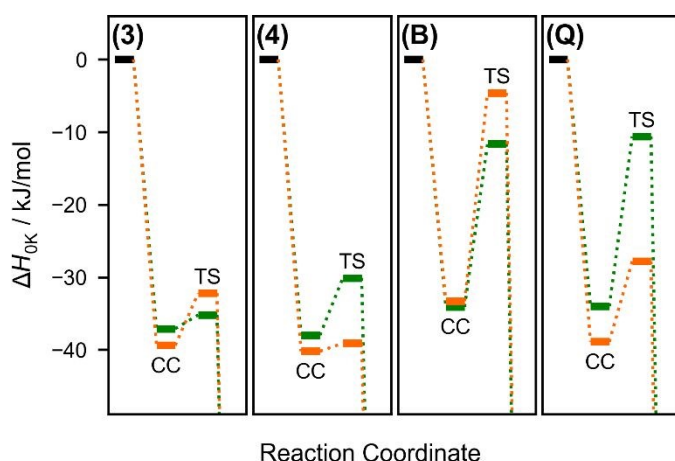
Figure 4: PES diagrams showing the OK reaction enthalpy for the formation of CC, TS and CA between ions 3 , 4 , B , and Q and MA (green paths) or ST (orange paths), calculated on M06-2X-D3/def2TZVPP level. Note that the CA states are not explicitly shown. CC = collisional complex, TS = transition state, CA = covalent adduct, MA = methyl acrylate, ST = styrene.
