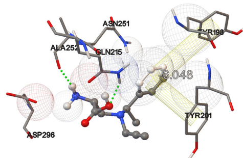
Fig. 3 Molecular docking analysis of the interaction between collagenase and ( S,S )-3-( N -(1-phenylethyl)- N -(prop-2-ynyl)amino)-2-aminopropanoic acid ( 4e ).
