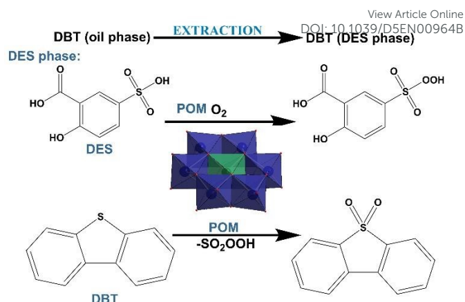
Figure 17. Schematic representation of the reaction mechanism for the oxidation desulfurization of DBT catalyzed by coupling \text{CrMo}_6 polyoxometalate with DESs under mild conditions ( T = 60^\circ\text{C} ). 284
