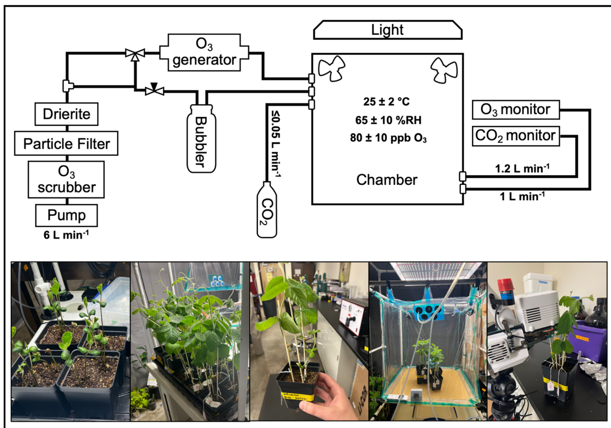
Fig. 1 Schematic of the custom-built plant fumigation chamber (top) and photos from the soybean vegetative growth cycle during the experiment (bottom). Total inlet flow of 6 L min -1 was split between the O_3 and humidification lines as needed to regulate RH and O_3 .
