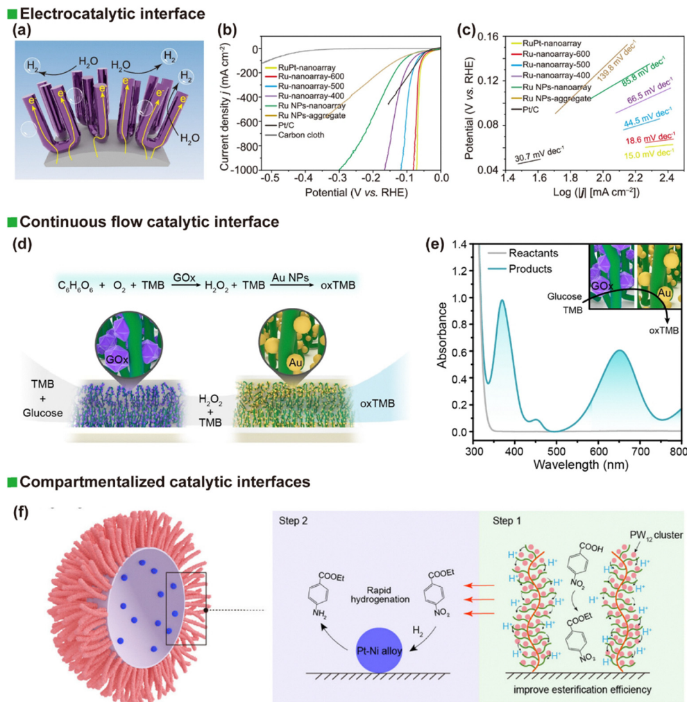
Fig. 17 (a) Schematic representation of a metallic Ru nanoarray designed for the hydrogen evolution reaction (HER). (b) iR-corrected polarization curves in 0.5 M H 2 SO 4 solution for alloy RuPt nanoarray, metallic Ru nanoarray- T , Ru NP nanoarray, Ru NP aggregates, commercial Pt/C-decorated carbon cloth, and pristine carbon cloth. (c) Tafel plots derived from the polarization curves shown in (b). Reproduced from ref. 54 with permission from Springer Nature, Copyright 2025. (d) and (e) Illustration and UV-vis spectra for a cascade reaction in PBS (pH 5.05) sequentially catalyzed by GOx-functionalized micellar brushes and Au NP-functionalized micellar brushes. Reproduced from ref. 51 with permission from Wiley, copyright 2021. (f) Schematic diagram of the sequential tandem conversion of p -nitrobenzoic acid within a microreactor engineered via surface modification strategies. Reproduced from ref. 55 with permission from Wiley, copyright 2025.
