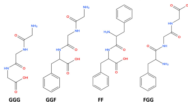
Scheme 2 Representative short-peptide structures: triglycine (glycylglycylglycine, GGG), diphenylalanine (L-phenylalanyl-L-phenylalanine, FF), phenylalanylglycylglycine (FGG) and glycyglycylphenylalanine (GGF), illustrating sequence variation used as model systems for analysing conformational control.
