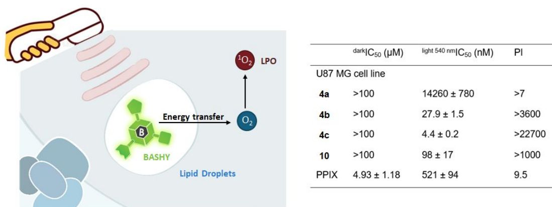
Figure 18. BASHY as a promising PS platform for PDT that targets LDs and triggers ferroptosis. Adapted from ref. 64 with permission from American Chemical Society, Copyright 2023.
