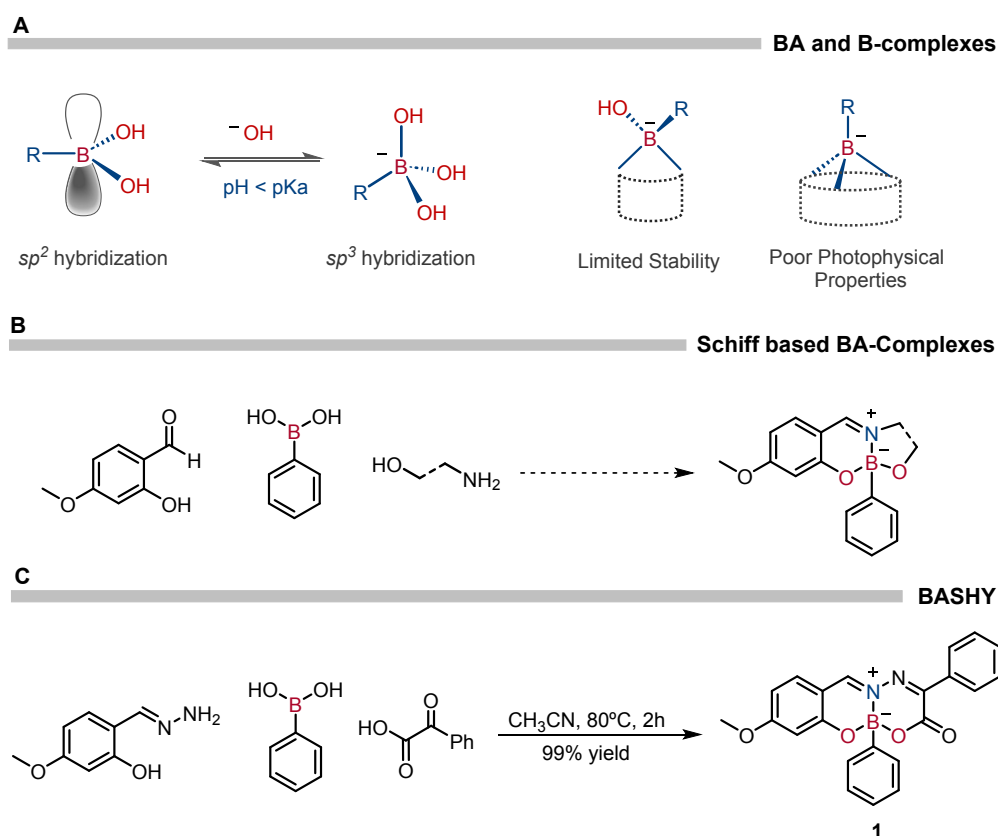
Figure 3. A) BA hybridization states and chelation with bi- and tri- dentate ligands; B) Schiff-base tetrahedral BA-complexes; C) Modular synthesis of BASHY dye 1 .
