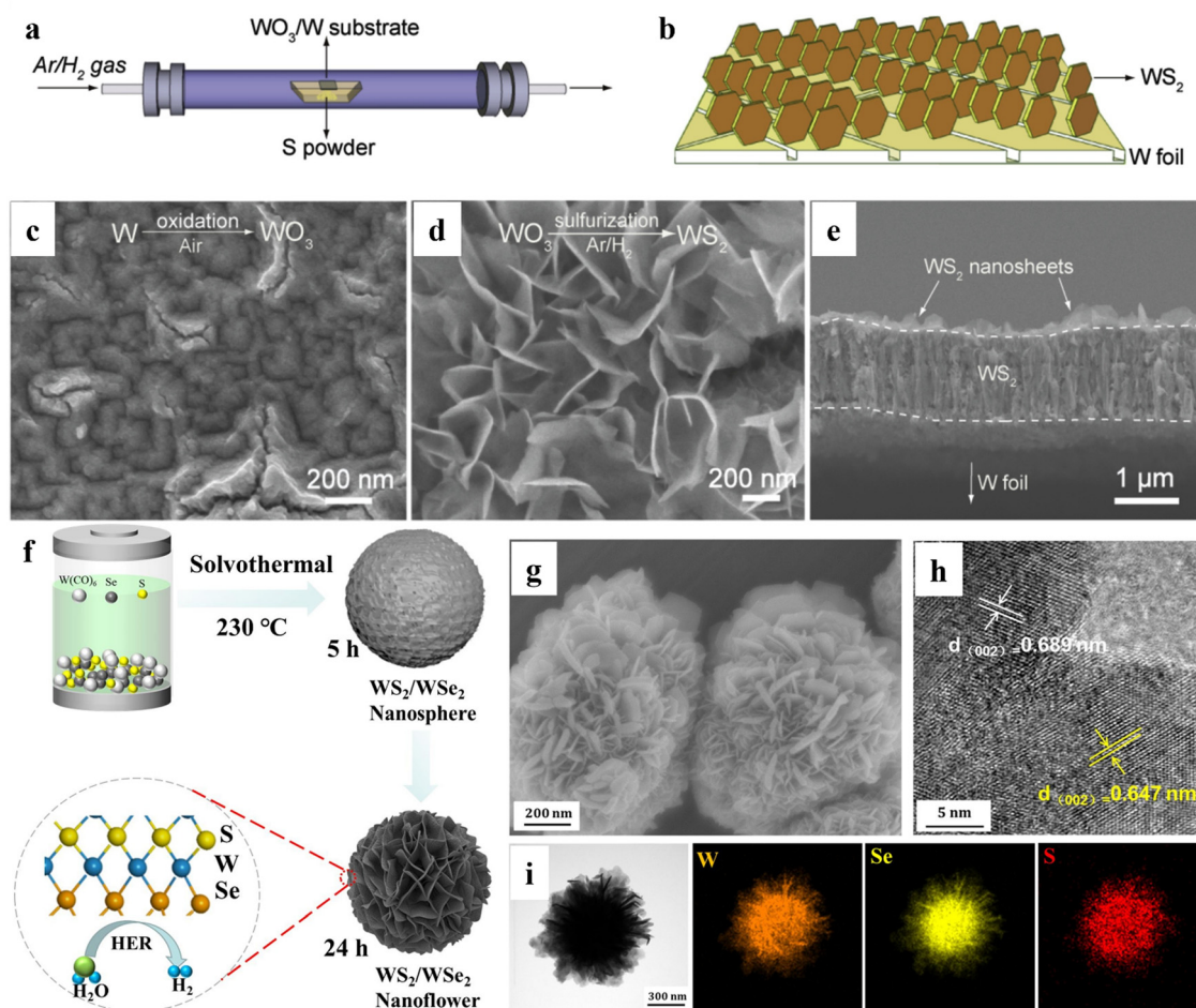
Fig. 3 (a) Schematic illustrating WS_2 synthesis process. (b) Structural diagram of WS_2/W . Scanning electron microscope (SEM) image of (c) WO_3 and (d) WS_2 nanosheets on W foil. (e) Side-view SEM image of WS_2/W . Reprinted with permission. 62 Copyright 2019, Elsevier. (f) Schematic illustration of the synthesis of the flower-like WS_2/WSe_2 heterostructure, (g) SEM image, (h) high resolution transmission electron microscope (HRTEM) image, and (i) high-angle annular dark-field scanning transmission electron microscope (HAADF-STEM) image of flower-like WS_2/WSe_2 heterostructure and energy dispersive X-ray spectroscopy (EDX) elemental mappings image. Reprinted with permission. 64 Copyright 2022, Elsevier.
