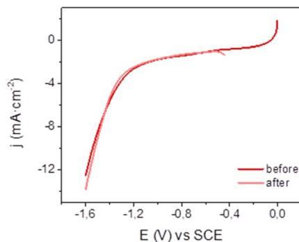
Fig. 7 Linear sweep voltammetry of Mn@Terpy-COF|NT ([Mn] total = 850 μmol cm -2 ) on CP at 10 mV s -1 before and after CPE at -1.3 V vs. SCE in water K 2 SO 4 /K 2 B 4 O 7 under CO 2 .
