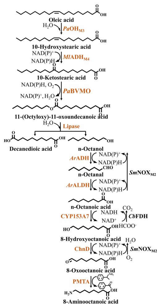
Fig. 5 Synthesis of 8-aminoctanoic acid from oleic acid. The abbreviations are as follows: PaOH M3 , mutant of oleic acid hydratase from Paracoccus aminophilus ; MIADH M4 , mutant of alcohol dehydrogenase from Micrococcus luteus ; PaBVMO, Baeyer–Villiger monooxygenase from Pseudomonas aeruginosa ; ArADH, alcohol dehydrogenase from Acinetobacter radioresistens ; ArALDH, aldehyde dehydrogenase from Acinetobacter radioresistens ; CYP153A, cytochrome P450 153A; ChnD, alcohol dehydrogenase; PMTA, ω-transaminase from Silicibacter pomeroyi .
