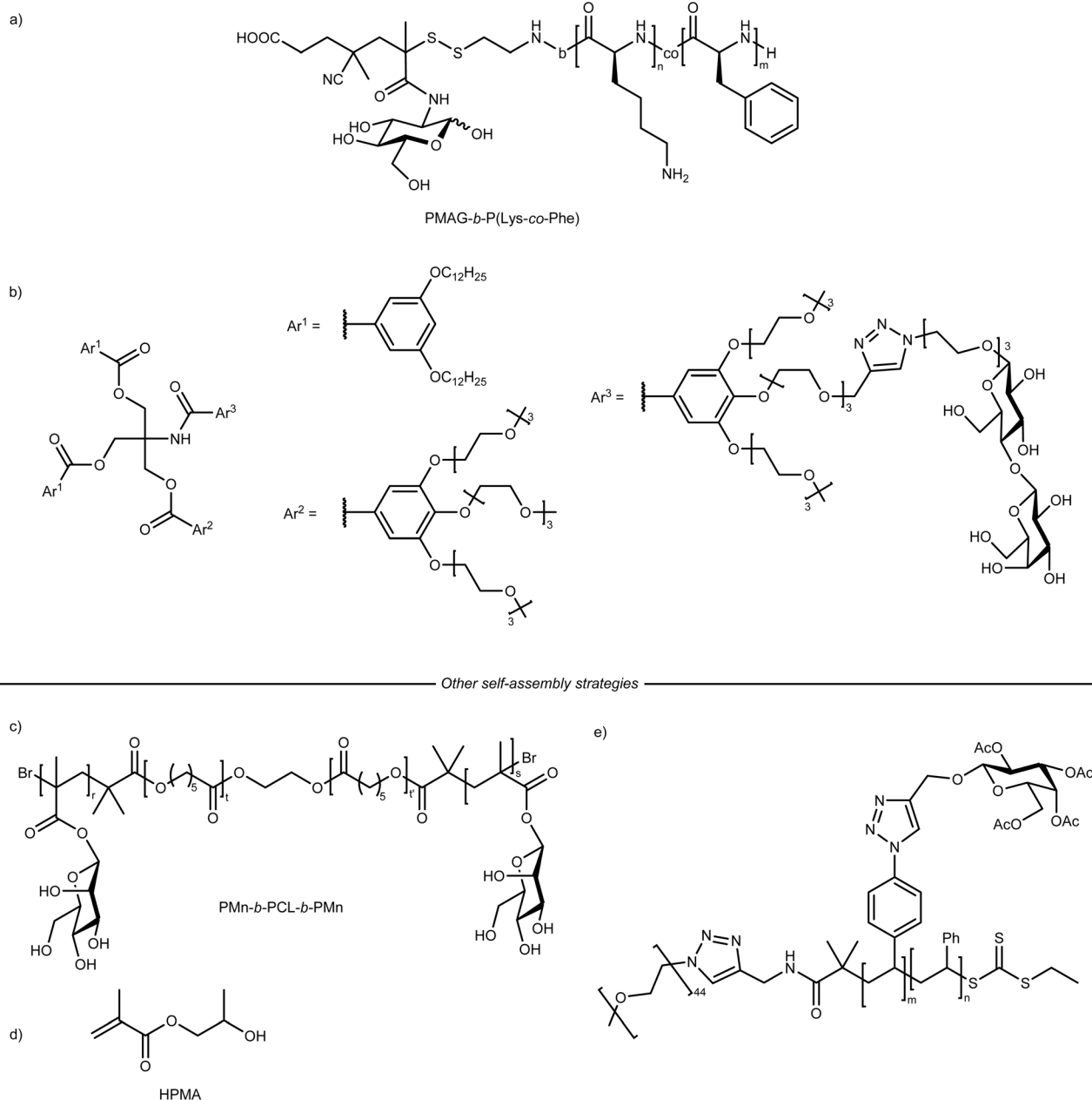
Fig. 4 Representative glycopolymer structures employed in the formation of glycopolymer-based nanoplatforms via self-assembly. (a) Structure of amphiphilic PMAG- b -P(Lys-co-Phe) copolymer forming spherical glycopolymer-based nanoplatforms; (b) structure of amphiphilic Janus glycodendrimers bearing sequence-defined oligomannose for the formation of glycodendrimersomes; (c) structure of mannose-mimicking ABA-type triblock copolymer (PMn- b -PCL- b -PMn), which electrostatically co-assembles with dihexadecyldimethylammonium bromide (DHDAB); (d) structure of hydroxypropyl methacrylate (HPMA) grafted onto dextran backbone, enabling UV-induced self-assembly into nanostructures; (e) representative glycopolymer structure applied in the "glyco-side" strategy.
