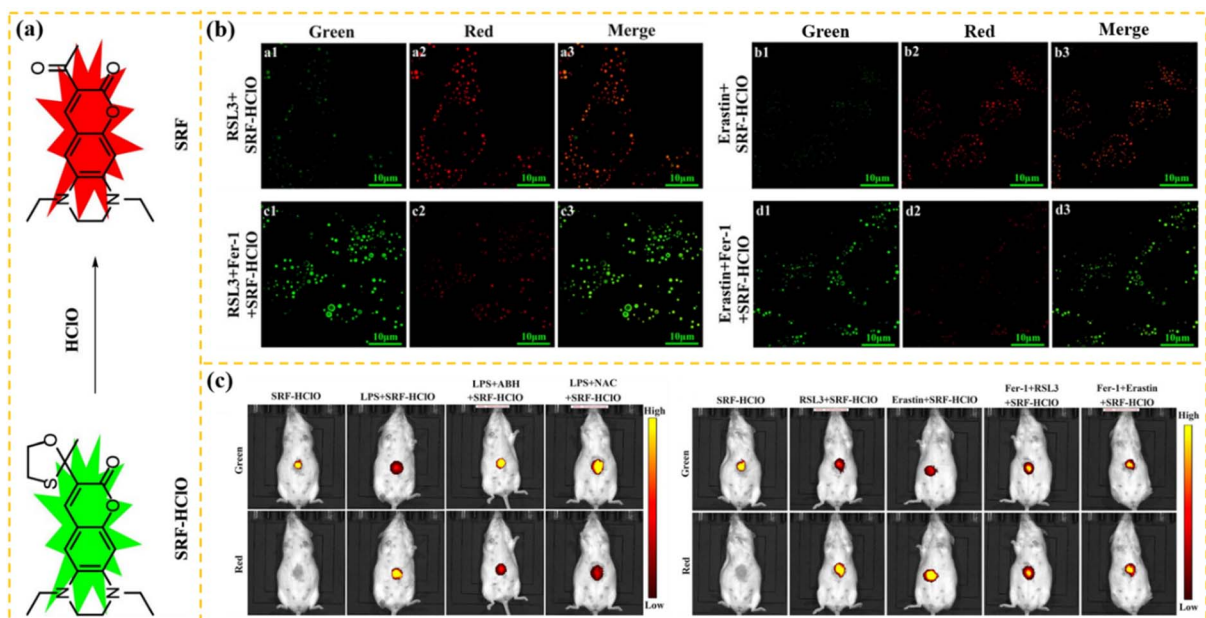
Fig. 44 (a) Chemical structure of probe SRF-HClO and the reaction mechanism of HClO. (b) Probe SRF-HClO is used for SIM imaging to detect cell HClO during different drug-induced ferrotosis processes. (c) SIM imaging of probe SRF-HClO in LPS-induced inflammation and different drug-induced ferrotosis mouse models. Reprinted with permission from American Chemical Society, copyright 2024, as cited in ref. 105.
