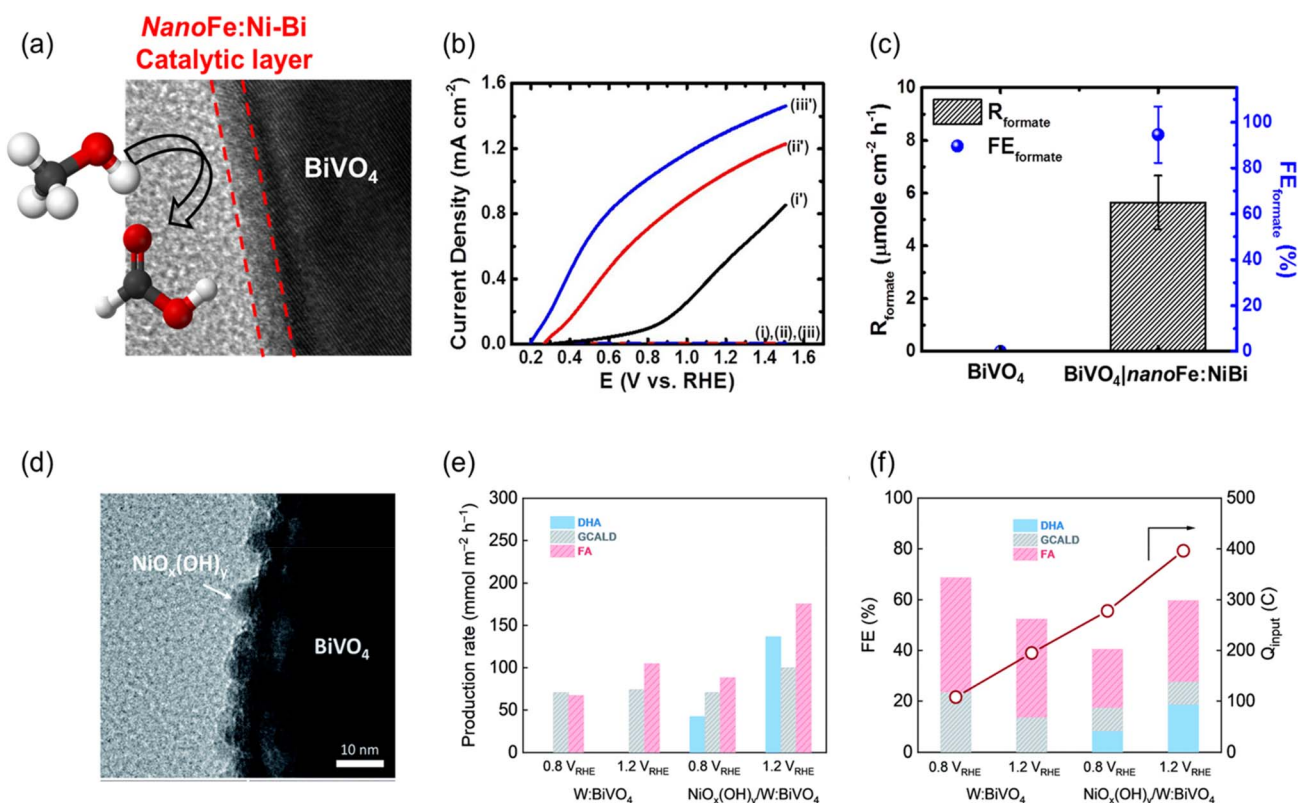
Fig. 11 (a) High-resolution transition electron microscopy (HRTEM) image shows the surface modification of the \text{BiVO}_4 photoanode with \text{nanoFe:Ni-Bi} . (b) LSV curves at a scan rate of 10 \text{ mV s}^{-1} of (i and i') the pristine \text{BiVO}_4 , (ii and ii') \text{BiVO}_4/\text{nanoFe:Ni-Bi} , and (iii and iii') \text{BiVO}_4/\text{nanoFe:Ni-Bi} photoanodes in near-neutral pH containing 0.1 M methanol in the dark (i'–iii') and under light illumination (i–iii). (c) Production rate of formate ( R_{\text{formate}} ) and \text{FE}_{\text{formate}} from PEC methanol oxidation using the pristine \text{BiVO}_4 and \text{BiVO}_4/\text{nanoFe:Ni-Bi} photoanodes. Reproduced with permission. 154 Copyright 2020, Elsevier. (d) HRTEM image illustrating \text{NiO}_x(\text{OH})_y co-catalyst incorporation on the surface of the \text{W:BiVO}_4 electrode. (e) Production rate and (f) FE with total charge passed ( Q_{\text{input}} ) obtained in 0.5 M KBI. Reproduced with permission under the terms of a CC BY-NC 3.0 license. 55 Copyright 2021, Royal Society of Chemistry.
