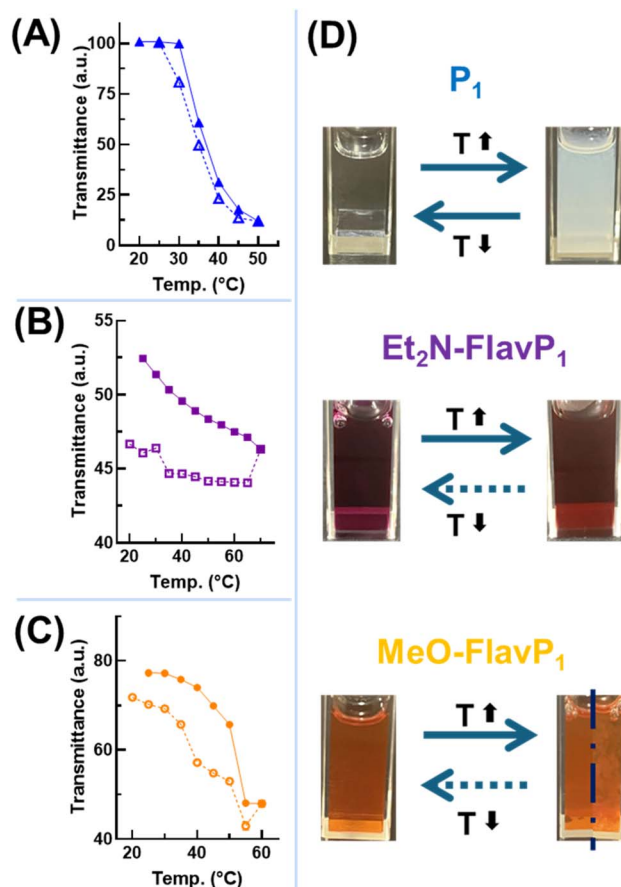
Fig. 5 Transmittance change at \lambda = 700 nm as a function of temperature of polymer solutions ( 1 \text{ g L}^{-1} ) of (A) parent polymer P 1 ; (B) Et 2 N-FlavP 1 and (C) MeO-FlavP 1 (solid line: heating; the dotted line: cooling); (D) states of polymeric solutions after heating: the heated MeO-FlavP 1 solution shows increased turbidity (left of blue line) and larger aggregates at 60 °C (right of blue line). On cooling, solid arrows indicate full transmittance recovery; dashed arrows indicate partial recovery.
