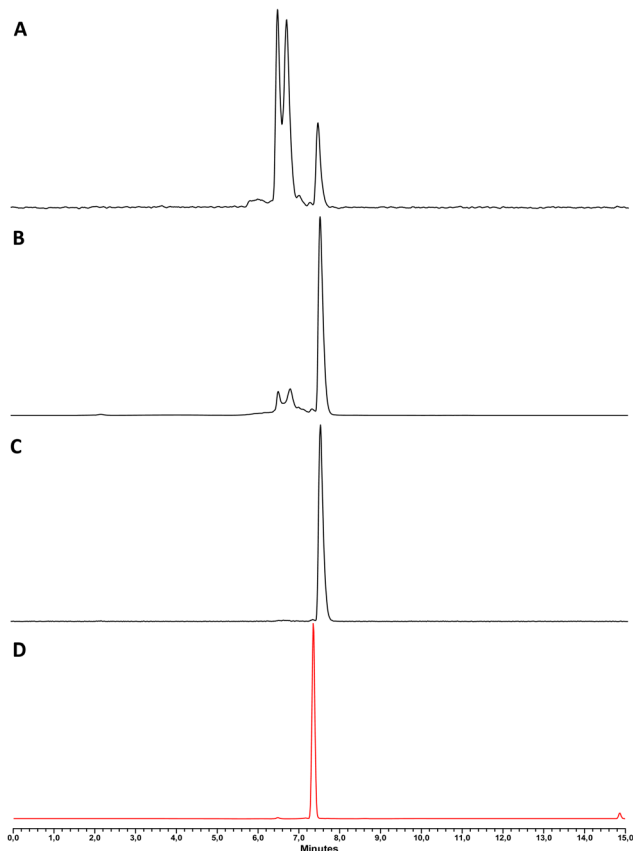
Fig. 7 Radio-HPLC chromatograms of (A) the unoptimised radiolabelling; (B) the optimised radiolabelling; (C) the final purified radiolabelling product, [^{188}\text{Re}]\text{ReO}(\text{N}_2\text{S}_2\text{-PEG}_3\text{-N}_3) and (D) UV chromatogram of ^{\text{nat}}\text{ReO}(\text{N}_2\text{S}_2\text{-PEG}_3\text{-N}_3) (358 nm).
