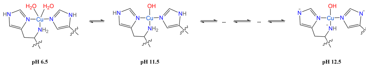
Scheme 2 Proposed species of SmAA10A at pH 6.5, 11.5 and 12.5 characterized by ^{1,2}\text{H} ENDOR spectroscopy.
