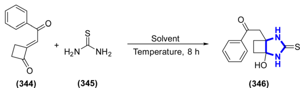
Scheme 95 Synthesis of 2-(phenylethylidene)cyclobutanones.
