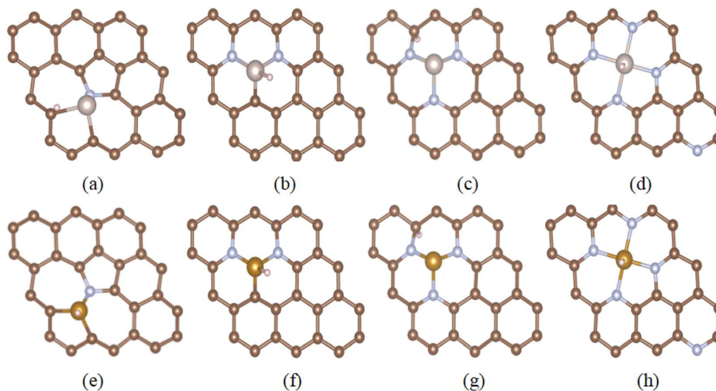
Fig. 6 The optimized hydrogen adsorption configurations at the most active sites on the (a) Ru SAC@N_pyrrolic, (b) Ru SAC@2N, (c) Ru SAC@3N, (d) Ru SACs@4N, (e) Fe SAC@N_pyrrolic, (f) Fe SAC@2N, (g) Fe SAC@3N and (h) Fe SAC@4N doped graphene. Dark brown, blue, gray, yellow and white represent C, N, Ru, Fe and H, respectively (side views are given in Fig. S7†).
