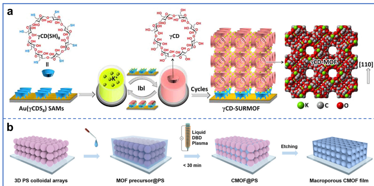
Fig. 3 (a) Preparation of \gamma\text{CD-SURMOF} membrane by assembly of metal ions and ligands layer by layer onto \gamma\text{CD(SH)}_8 modified Au substrates. Reproduced with permission from ref. 29. Copyright 2022, Chinese Chemical Society. (b) Preparation of M-CMOF membranes with hierarchical porous structures by using PS arrays as templates. Reproduced with permission from ref. 30. Copyright 2024, American Chemical Society.
