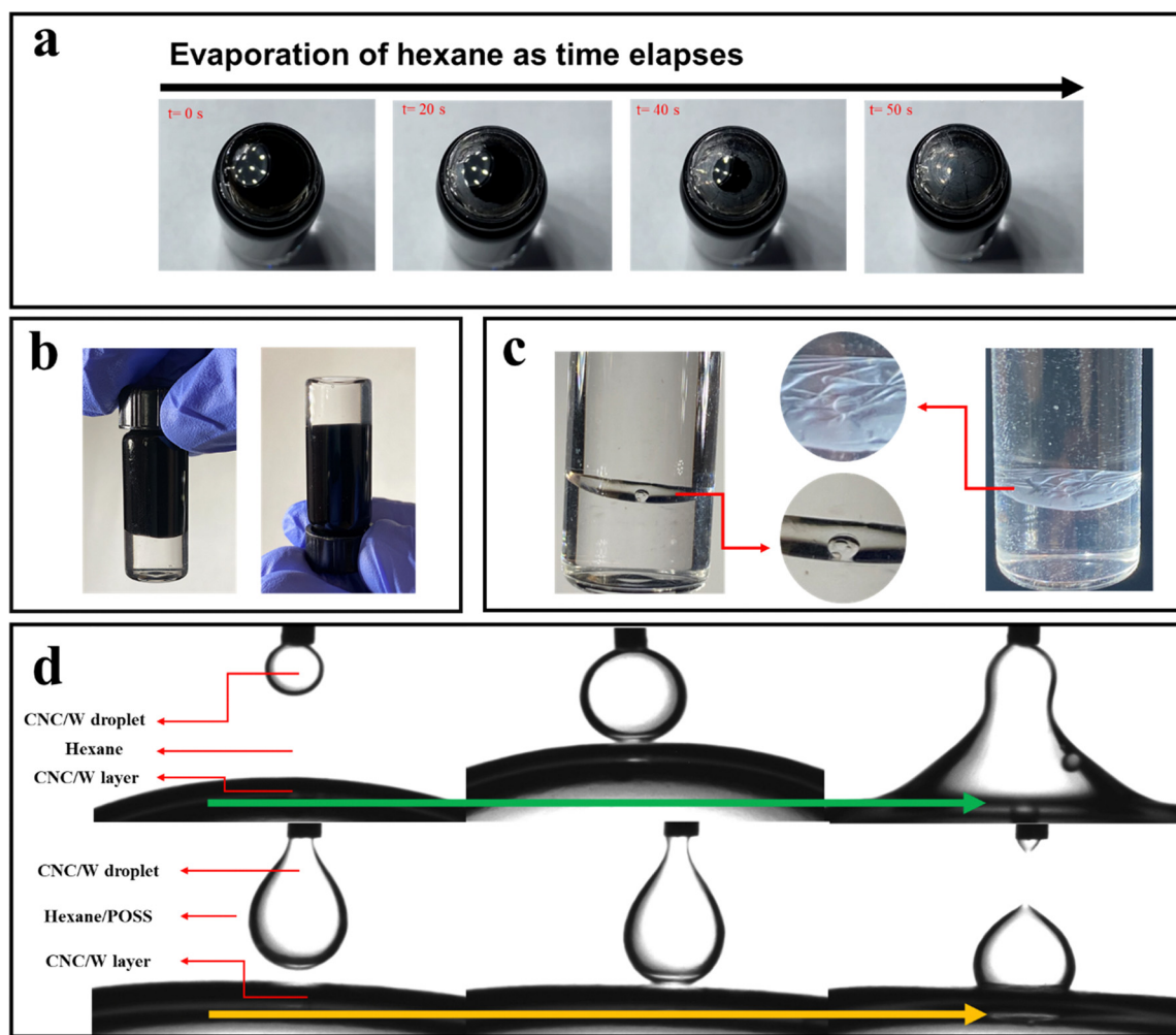
Fig. 2 (a) GO-POSS NPSs layer formation during hexane evaporation, with the layer generation process lasting approximately 50 seconds in a vial (width \approx 16.4 mm, height \approx 47.6 mm). (b) Compartmentalized all-aqueous GO and CNC suspensions in a vial (width \approx 16.4 mm, height \approx 47.6 mm). (c) CNC suspension droplet stability on top of the CNC suspension/hexane-POSS interface immediately after interface formation and after a week in a vial (width \approx 24.6 mm, height \approx 48.4 mm). (d) Droplet stability at the interface of CNC suspension/hexane in the presence (bottom) and absence (top) of POSS in the hexane phase, process lasting approximately 45 seconds.
