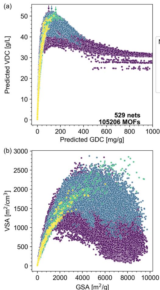
Fig. 9 Analysis of MOF data points colored by net density. (a) Scatter plot comparing predicted VDC versus predicted GDC, color-coded into four subgroups by net density: purple (0–1), blue (1–2), green (2–3), and yellow (>3). The peak performance of each subgroup is indicated with a color-matched arrow except for yellow (>3). (b) Scatter plot comparing VSA versus GSA, with the same color scheme. Higher density MOFs are plotted on the top. Fig. S28–S31† show the data points of subgroups separately.
