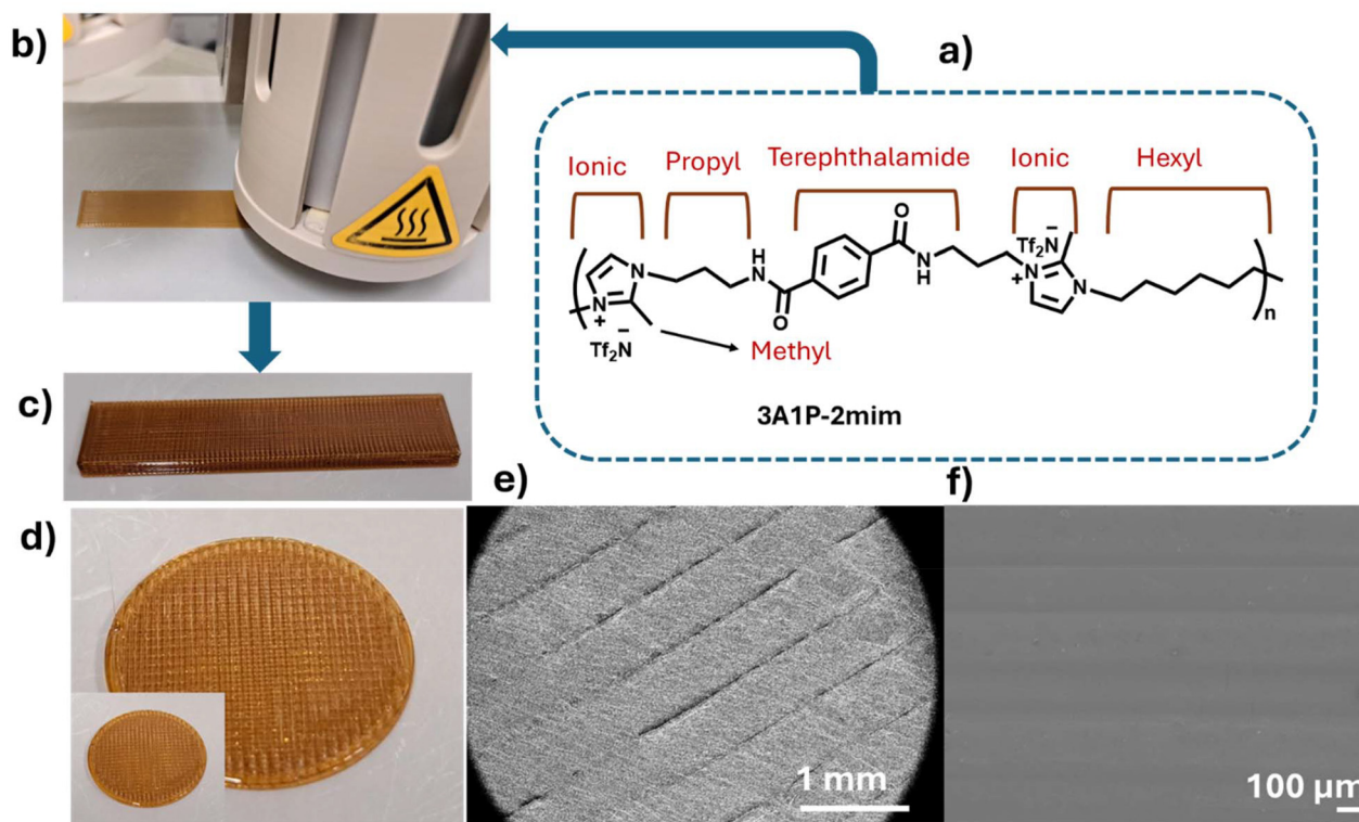
Fig. 5 (a) Repeat unit structure and segments of 3A1P-2mim PA-ionene contributing intramolecular interaction. (b) 3D printing of first two layers of a slab ( \sim 0.66 mm thickness at this point). (c) Completed slab (9 layers, \sim 2.88 mm thickness). (d) 3D printed disc (5 layers, 1.2 mm thickness). (e) SEM infill pattern orientation for 3D printed slabs and discs. (f) Stretching was observed in the SEM image of the slab after tensile testing.
