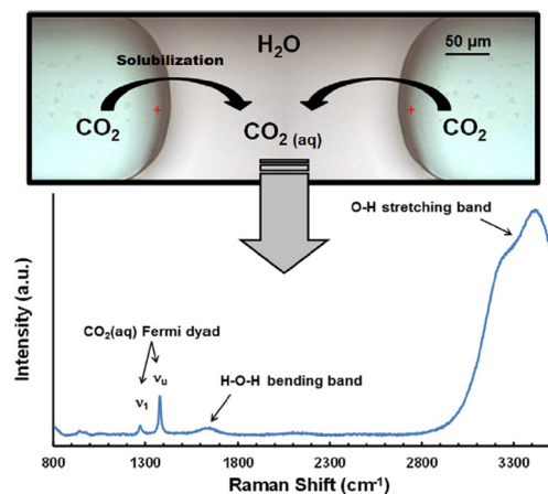
Fig. 12 Optical image of a CO 2 –water flow inside a microchannel and corresponding confocal Raman spectra within a water slug containing dissolved CO 2 . Reproduced from Liu et al. 117 with permission from Elsevier, copyright 2012.
