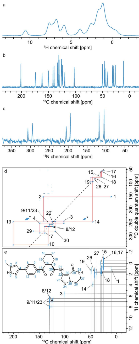
Fig. 11 Spectra used for the carbon-13 detection based assignment of Atuliflapon (chemical structure shown inset). ^{54} One dimensional (a) ^1\text{H} (21.1 T, 111 kHz MAS rate, 298 K), (b) ^{13}\text{C} CP (11.7 T, 22 kHz MAS rate, 298 K) and (c) ^{15}\text{N} CP (9.4 T, 12 kHz MAS rate, 298 K) NMR spectra. (d) ^{13}\text{C} - ^{13}\text{C} DNP enhanced solvent suppressed INADEQUATE (9.4 T, 12.5 kHz MAS rate, 100 K), and (e), ^1\text{H} - ^{13}\text{C} HETCOR spectra (11.7 T, 22 kHz MAS rate, with eDUMBO- 1_{22} homonuclear decoupling ^{236} in t_1 ). In (d), the ^{13}\text{C} peaks denoted by an asterisk at 60 and 170 ppm are attributed to impurities introduced during sample preparation. Adapted from ref. 54.
