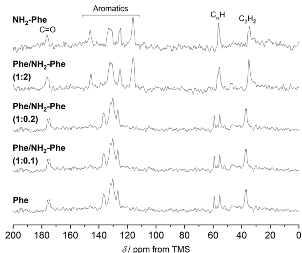
Fig. 9 ^1\text{H} - ^{13}\text{C} CP/MAS NMR spectra of Phe (303 mM), Phe/ \text{NH}_2 -Phe (1 : 0.1), Phe/ \text{NH}_2 -Phe (1 : 0.2), Phe/ \text{NH}_2 -Phe (1 : 2) and \text{NH}_2 -Phe (606 mM) hydrogels acquired with an MAS rate of 8.5 kHz using a 400 MHz solid-state NMR spectrometer.
