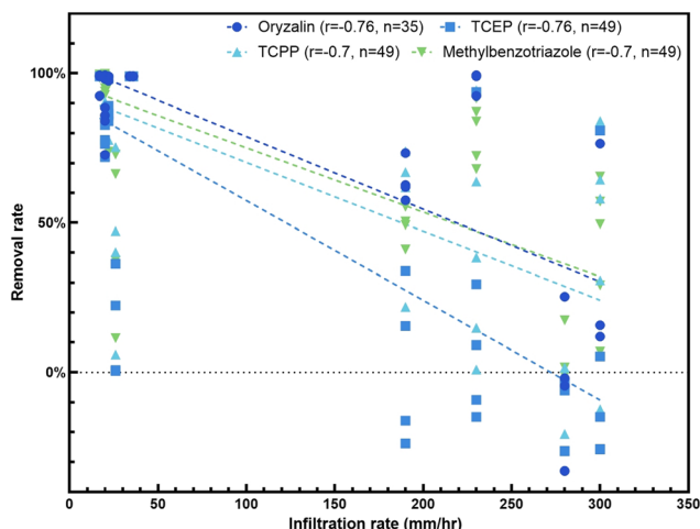
Fig. 6 The impact of infiltration rate towards biofiltration systems performance for four organic chemicals (oryzalin, TCEP, TCP, methylbenzotriazole).
