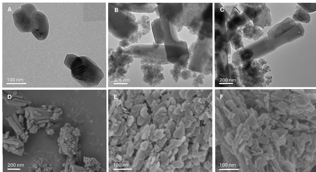
Fig. 6 Electron micrographs of dispersed hydroxyapatite particles isolated from bovine bones following different treatments. A) High-resolution TEM micrograph of HAC (magnification of 120 k), highlighting merged grain boundaries; B and C) high-resolution TEM micrograph of HAcM (magnification of 120 k) highlighting fractal-like agglomerates of ultrafine amorphous particles and broken or strained nanorods; D) SEM micrograph of HAcM (magnification of 40 k) displaying the morphological and size heterogeneity; E and F) SEM micrographs of HAK and HAW (magnification of 100 k), revealing nano-platelets less heterogeneous in morphology and size compared to HAcM.
