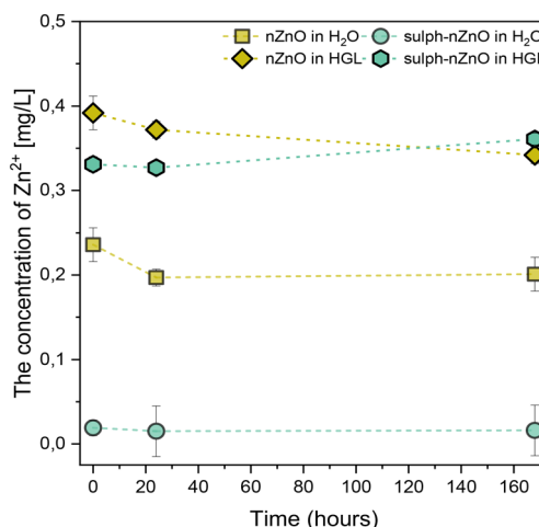
Fig. 2 The concentration of \text{Zn}^{2+} in MQ water and Hoagland medium (HGL) with nZnO and sulph-nZnO at a rate of 0.05 Zn per L measured after 0, 1, and 7 days. The concentration of \text{Zn}^{2+} was determined by the ICP-OES instrument in the previous filtered solutions using Microsep Advance centrifugal devices with omega membrane 1 K. Error bars represent standard error ( n = 3 repeats).
