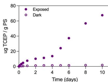
Fig. 3 Concentration of TCEP detected in the leachate of a 1 w/w% TCEP-PS composite suspended in water and exposed to UV_{>300\text{nm}} irradiation (closed circles) or under dark conditions (open circles).
