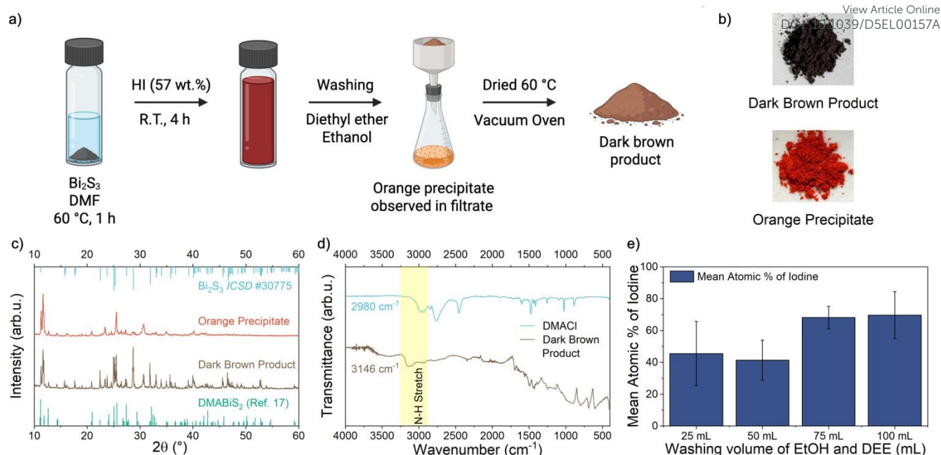
Figure 2. Preparation of DMABiS 2 Intermediate. (a) Illustration of the synthesis procedure for preparation of the DMABiS 2 intermediate. Created in BioRender. Quinn, E. (2025) https://BioRender.com/xo6o9y9 (b) Images of the dark brown product powder and the orange precipitate observed in the filtrate during the washing stage. (c) PXRD pattern of synthesized DMABiS 2 material. The light blue bars indicate the reference patterns of Bi 2 S 3 (ICSD #30775), while the light green bars represent the reported pattern by Huang et al. for their claimed DMABiS 2 intermediate. (d) Infrared spectra of the dark brown powder and DMABiS 2 reference material. The peaks assigned to the ammonium N-H stretch are highlighted. The increase in peak wavenumber for the dark brown powder sample is attributed to the reduction in electronegativity of the environment leading to stronger N-H bonds. (e) The effect of solvent washing volume on the mean atomic percentage of iodine from EDS measurements of dark brown product powders. The error of atomic percentage is calculated using procedure described in Fig. S12, SI.
