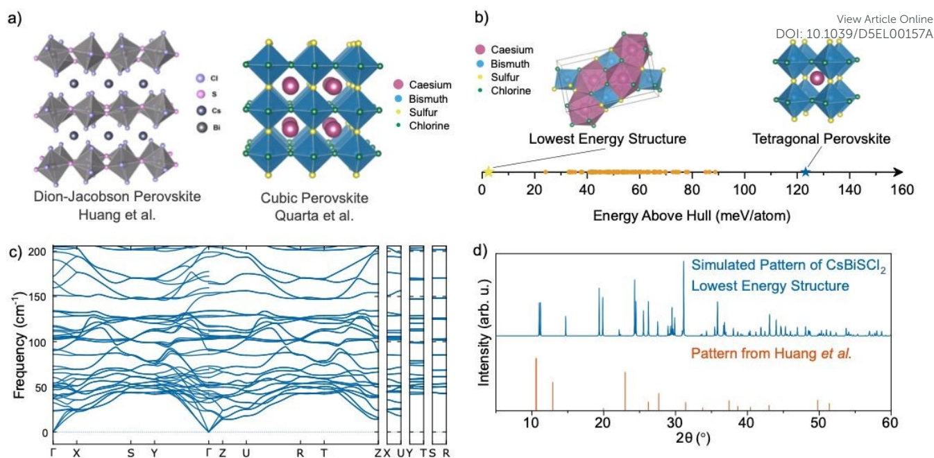
Figure 1. Structure of CsBiSCl 2 (a) Proposed crystal structure of CsBiSCl 2 by Huang et al. 17 and Quarta et al. 33 Illustration of structure proposed Huang et al. reprinted with permission from J. Huang et al. , J. Phys. Chem. Lett. , 2024, 15 , 3383–3389. Cubic perovskite structure prepared from the information provided in Ref. 33. (b) Energy above the Cs-Bi-S-Cl convex hull of CsBiSCl 2 structures selected for DFT refinalization. Shown are the lowest energy structure (yellow star), tetragonal perovskite structure (blue star), and remaining CsBiSCl 2 structures within 70 meV/atom of the hull (orange circles). (c) Phonon dispersion curve of the lowest-energy CsBiSCl 2 structure found from AiRSS. Lack of imaginary modes ( i.e. , no negative frequencies) demonstrates the dynamic stability of this structure. (d) Comparison of the simulated powder X-ray diffraction (PXRD) pattern for the lowest energy Pnma structure and the CsBiSCl 2 PXRD pattern reported by Huang et al. 17 Comparison with tetragonal perovskite reference pattern shown in Fig. S6, SI.
