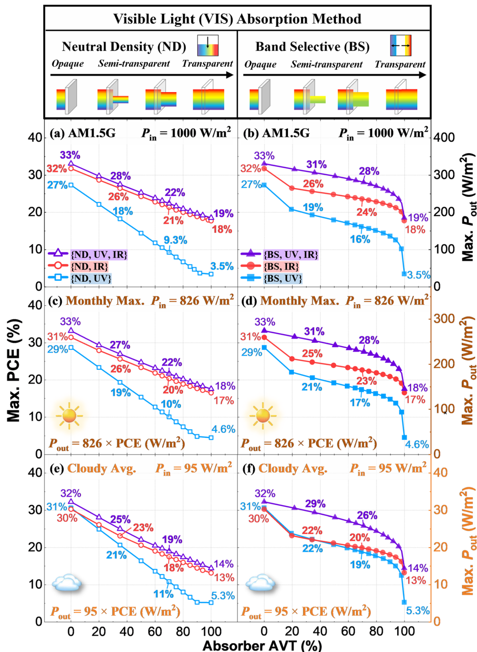
Fig. 7 The Shockley–Queisser-limit PCE (left axes) and the corresponding max. P_{\text{out}} (right axes) vs. absorber AVT under the AM 1.5G (top row, a and b), monthly max. (centre row, c and d), and cloudy avg. (bottom row, e and f) irradiance conditions using the neutral density (ND, left panel, a, c and e) and the band selective (BS, right panel, b, d and f) methods. The harvestable power intensity ( P_{\text{in}} ) and the corresponding max. P_{\text{out}} are stated in each row of irradiance conditions. In each subfigure, the colors and symbols represent the three INVIS absorption modes (UV + IR: purple triangles; IR: red circles; UV: blue squares), with the max. PCE values annotated for specific AVT levels (0% opaque, 35% translucent, 70% highly transparent, 100% fully transparent). The corresponding max. P_{\text{out}} values are tabulated in Table 1. Within each row, the harvestable irradiance spectra of the ND and BS methods at 0% and 100% absorber AVT are identical, respectively. The {ND, UV, IR} curve in (a) mimics the ‘wavelength-selective’ strategy 26 up to the range of wavelength. Note the same max. PCE scales (left axes) but distinct max. P_{\text{out}} scales (right axes) across the rows.
