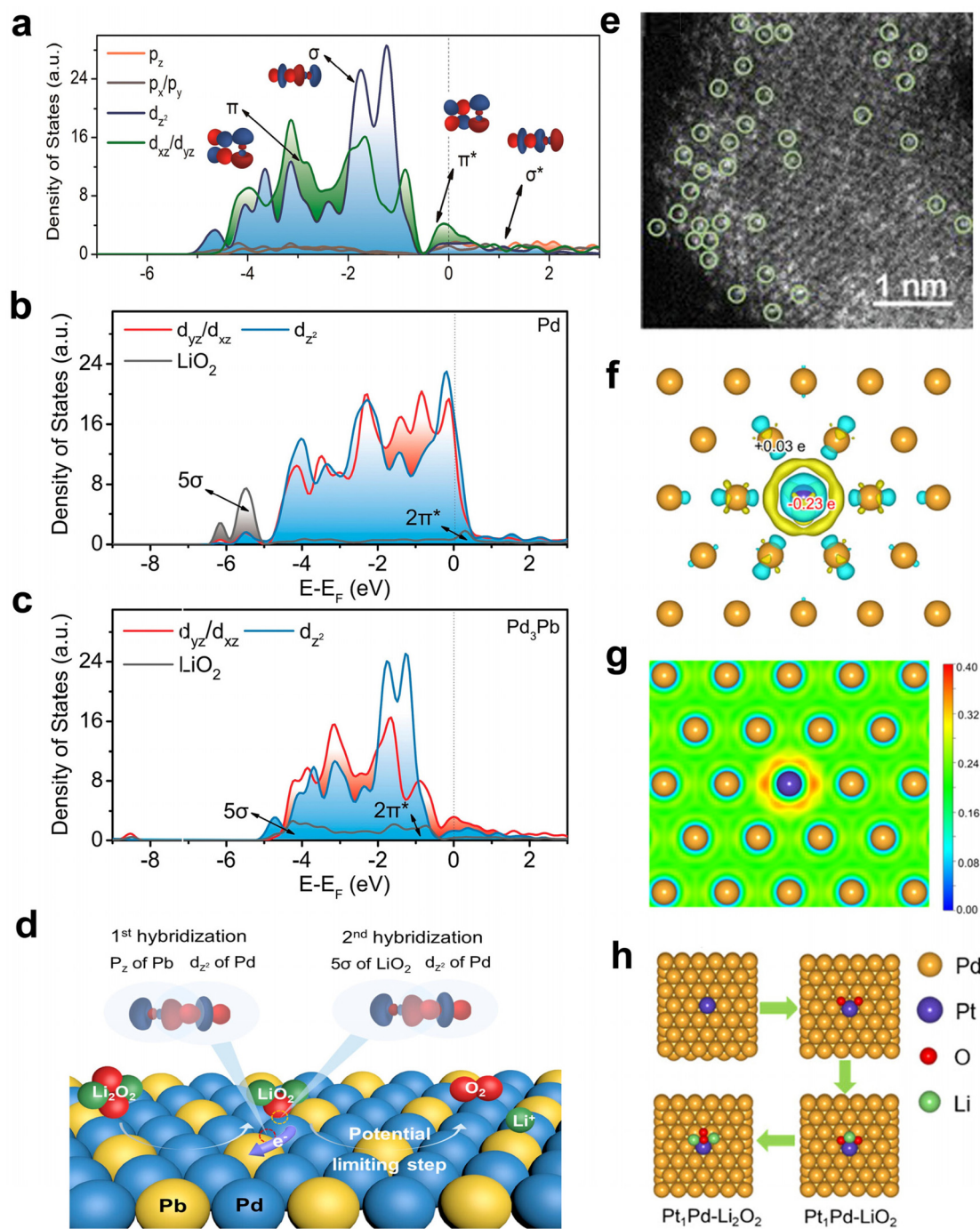
Fig. 13 (a) DOS of Pd d_{z^2} , d_{xz/yz} orbitals and Pb p_x , p_y , p_z orbitals after intra-molecular p-d orbital hybridization in Pd 3 Pb. (b) DOS of Pd 4d d_{yz/d_{xz}} , d_{z^2} orbitals in Pd. (c) DOS of Pd 4d d_{yz/d_{xz}} , d_{z^2} orbitals in Pd 3 Pb with adsorbed LiO 2 . (d) Schematic representation of cascade orbital-oriented hybridization from intra-molecular Pb-Pd p-d hybridization in Pd 3 Pb to inter-molecular orbital hybridization between Pd 3 Pb (Pd 4d xz/yz and 4d z 2 ) and LiO 2 (2π* and 5σ), using the d z 2 orbital along the z-axis as an example. 115 (e) AC-HAADF-STEM image of the Pt 1 Pd alloy (single-atom Pt marked with green circles). (f) ELF values of Pt 1 Pd. (g) Charge density difference distribution (regions of electron enrichment and depletion) in Pt 1 Pd. (h) Schematic representation of the discharge pathway of a Li-O 2 battery on the Pt 1 Pd surface. 40
