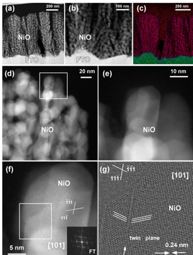
Fig. 7 (a) Low magnification HAADF-STEM cross-sectional image for a specimen grown at 100 °C. (b) Low magnification HAADF-STEM image of NiO/FTO interface. (c) EDXS-STEM elemental map showing Ni, O, and Sn distribution (color codes: Ni, red; O, blue; Sn, green). (d) Middle magnification micrograph of the outermost material region, and (e) high magnification HAADF-STEM micrograph of NiO grains framed by the white box in (d). (f) High resolution [101] HAADF-STEM image of NiO grain in (e) and corresponding Fourier transform (FT) pattern. (g) Magnified [101] HAADF-STEM image of the region selected by the white frame in (f). Twin \langle 111 \rangle planes are evidenced by a white arrow, and the distance between \langle 111 \rangle planes is marked.
