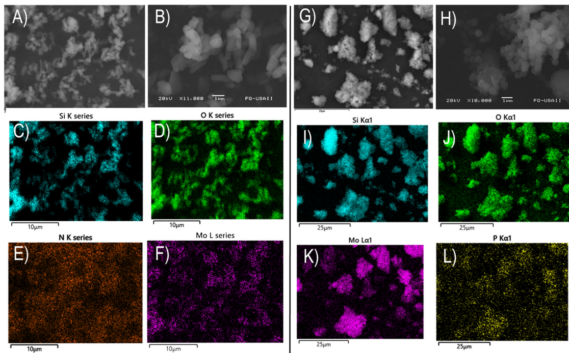
Fig. 2 SEM micrographs of as-synthesized materials. SBA-15-[PEIH] x [PMo 12 O 40 ] (low-magnification (A), high-magnification (B)), EDS element mapping of Si (C), O (D), N (E) and Mo (F) and Stöber-[PEIH] x [PMo 12 O 40 ] (low-magnification (G), high-magnification (H)), EDX element mapping of Si (I), O (J), Mo (K) and P (L).
