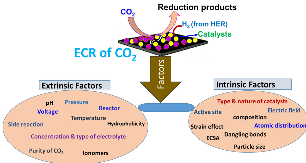
Fig. 6 Extrinsic and intrinsic factors affecting the ECR of \text{CO}_2 .
