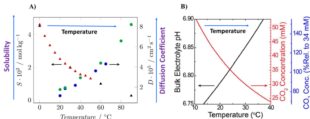
Fig. 19 (A) Dependence of CO 2 solubility (S) in 2 M aqueous NaCl solution (triangles, black: red) and CO 2 diffusion coefficient in water (circles, blue, green) temperature effect on electrolyte, 200 (B) effect of temperature on the equilibrium pH (black) and equilibrium dissolved CO 2 concentration (red) obtained for a 0.1 M NaHCO 3 electrolyte in equilibrium with 1 atm of CO 2 . The far right hand axis (blue) shows the dissolved CO 2 concentration normalized to the value for 25 °C. Reproduced with permission. 146 ©The Royal Society of Chemistry.
