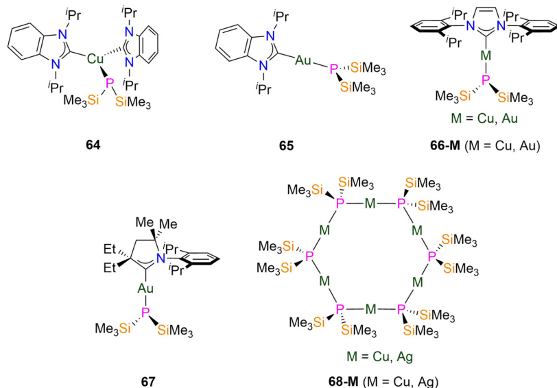
Fig. 19 Group 11 P'' complexes [Cu(iPr_2\text{-bimy})_2(P'')] 64 ( iPr_2\text{-bimy} = 1,3-di-isopropylbenzimidazole-2-ylidene), [Au(iPr_2\text{-bimy})(P'')] ( 65 ); [M(iPr)(P'')] ( 66-M ; M = Cu, Au ), iPr = (1,3-bis(2,6-diisopropylphenyl)-2-ylidene), [Au(CAAC^{MeEt})(P'')] ( 67 , CAAC^{MeEt} = dimethyl-diethyl-cyclic(alkyl)(amino)carbene), [M(\mu-P'')]_6 ( 68-M ; M = Cu, Ag ).
