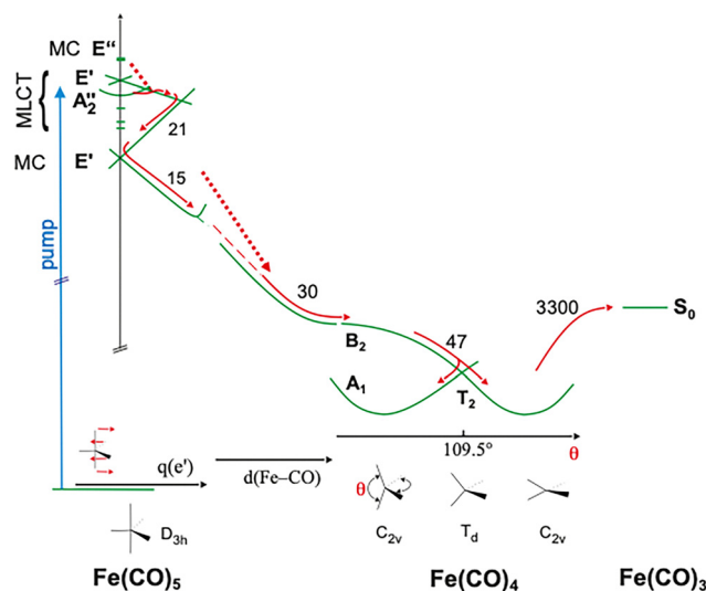
Fig. 5 Suggested potentials and paths for Fe(CO) 5 photodissociation, with our previously measured 33 time constants (in fs). The sequence of excited states qualitatively follows the calculation of Malcomson et al. , 2 though the energetic distance of A 2 ' and E' (nearly degenerate in the calculation) is enlarged for reasons of visibility. Pseudorotation is denoted q(e') in the parent molecule and \theta in Fe(CO) 4 . For the times up to dissociation, two paths are suggested: the solid arrows (preferred in the text) lead via the lowest MC state, whereas the (interrupted) dotted arrow would lead around a crossing with the steeply descending potential from the higher MC E'' state; this latter path would be analogous to Cr(CO) 6 , shown in Fig. 4. For the CoIn in Fe(CO) 4 , we (as others) assumed tetrahedral geometry (T d ) and a triply degenerate electronic state (T 2 ); Paterson et al. point out that their calculations predict a degenerate (E) and a nondegenerate (A 1 ) state lying nearby, which may influence details of the relaxation path. 23 – Elimination of a second CO, which is due to excess energy in the primary product and occurs on a picosecond time scale, is shown for completeness but is not discussed in the text.
