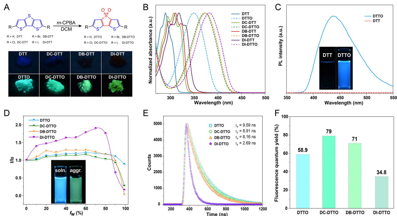
Fig. 2 (A) Synthetic route and molecular structures of DTTs with halogen substitution. (B) UV-vis spectra of DTTs and DTTOs. (C) PL spectra of DTT and DTTO in THF solution. (D) Plots between the ratio of I/I_0 and water fraction in H_2O/THF mixtures; I_0 and I are the maximum PL intensity of DTTOs in pure THF and in H_2O/THF mixtures (concentration: 1 \times 10^{-5} \text{ mol L}^{-1} ), respectively; inset: fluorescence photograph of DI-DTTO in pure THF and in 99% H_2O/THF mixtures taken under 365 nm UV irradiation. (E) Fluorescence lifetimes, and (F) fluorescence quantum yields of DTTOs in THF solutions.
